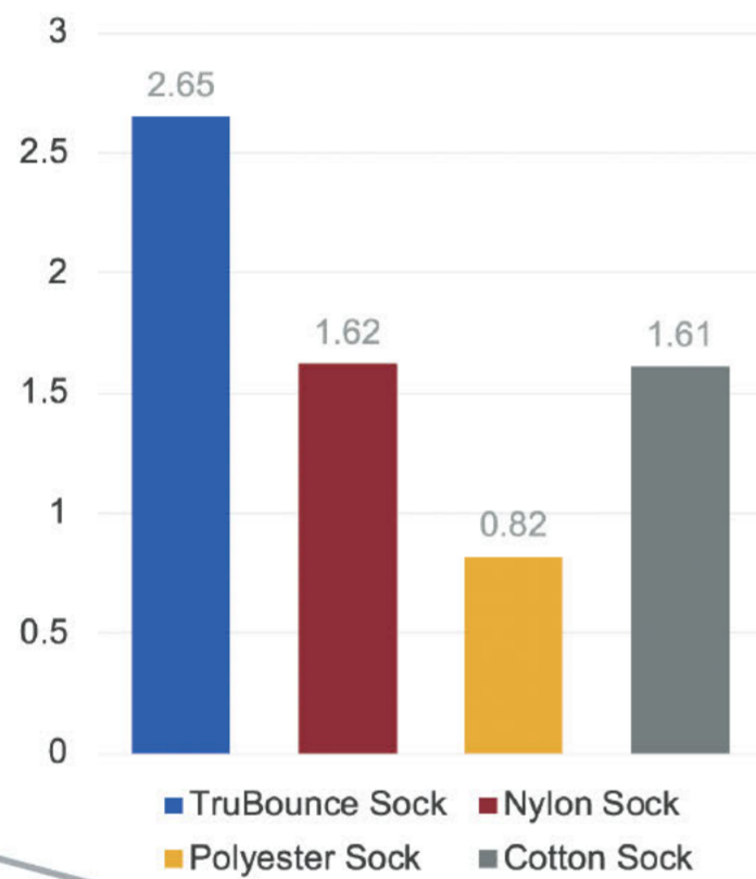
FORCE REQUIRED FOR 25% COMPRESSION
