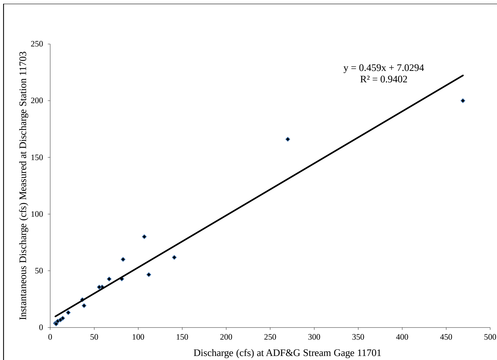
Figure 5.—Simple Linear Regression model used to estimate relationship between discharge station 11703 and streamgage 11701.
