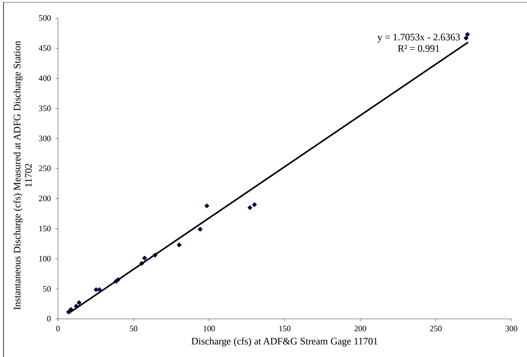
Figure 4.—Simple Linear Regression model used to estimate relationship between discharge station 11702 and streamgage 11701.
