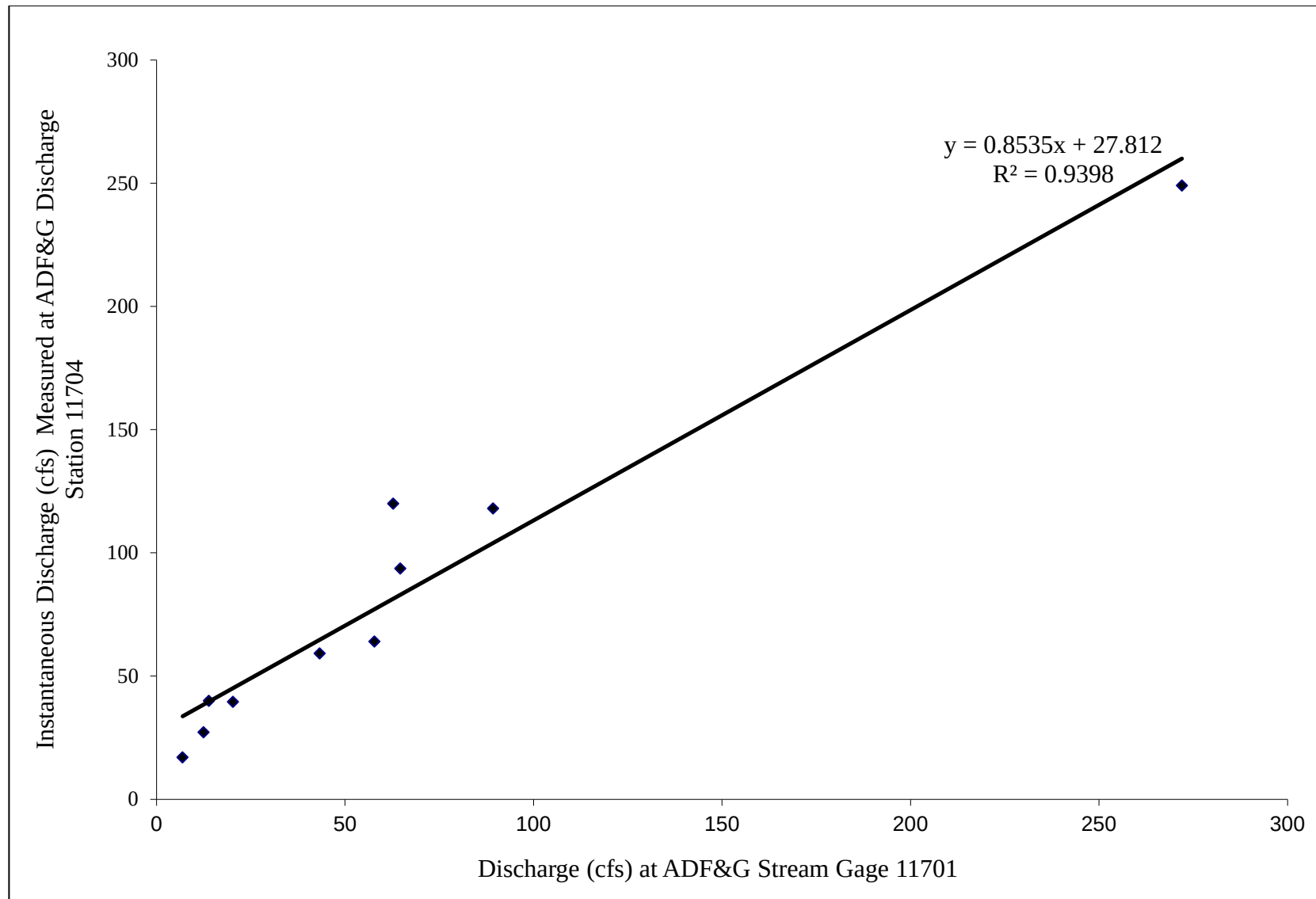
Figure 6.—Simple Linear Regression model used to estimate relationship between discharge station 11704 and streamgage 11701.
