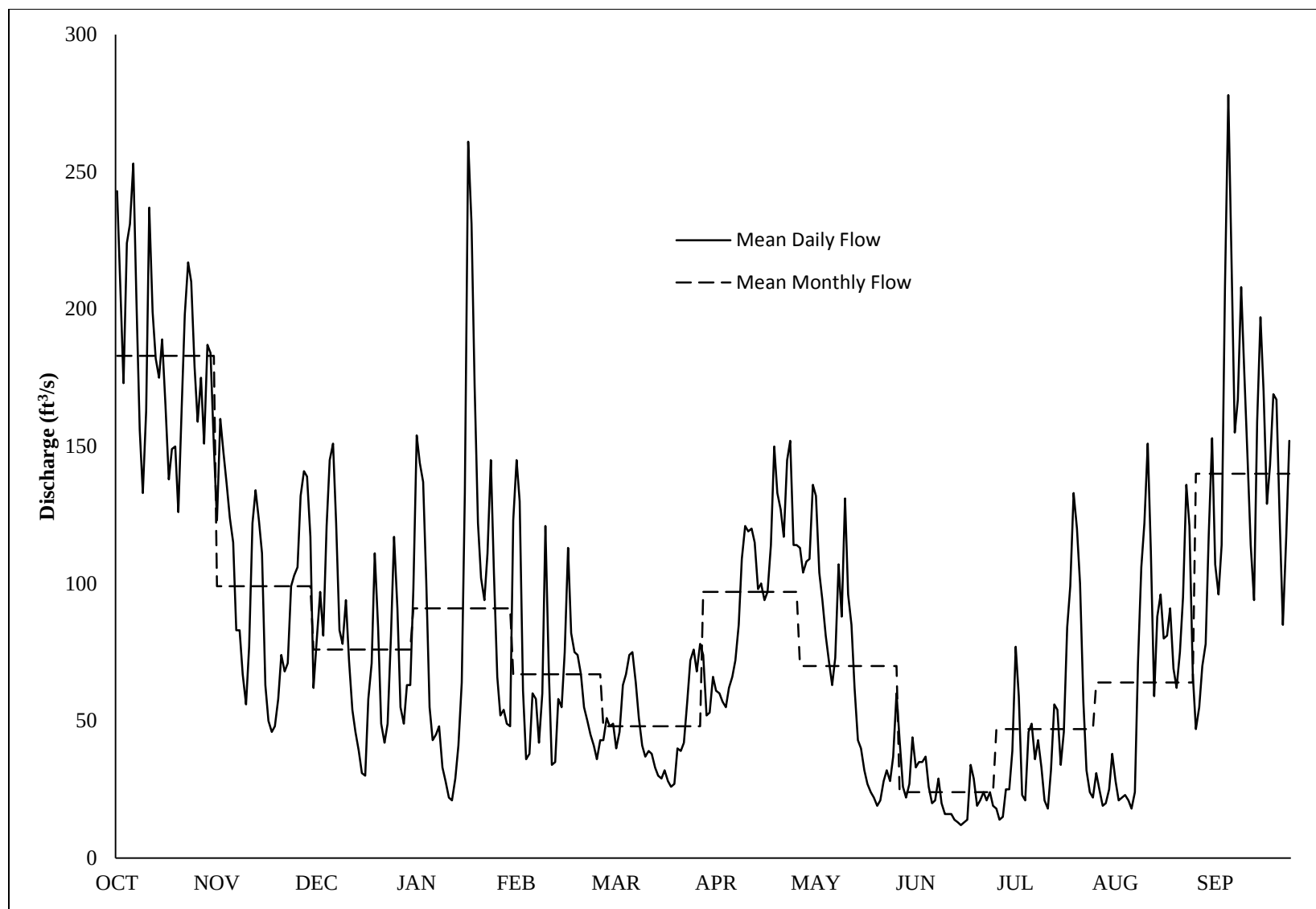
Figure 3.—Mean daily (October 1, 2006 to September 30, 2011) and mean monthly (October 1, 2006 to September 30, 2011) flows for the Lost River, Southeast Alaska, based on data from streamgage 11701.
