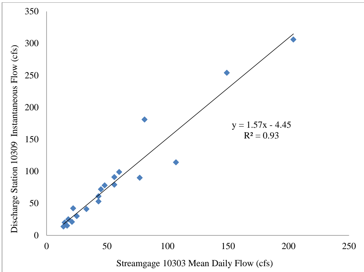
Figure 5.—Simple Linear Regression model used to estimate relationship of streamflows between discharge station 10309 (located in Reach A near the mouth of Sitkoh Creek) and streamgage 10303 (located in Reach B at the outlet of Sitkoh Lake).
