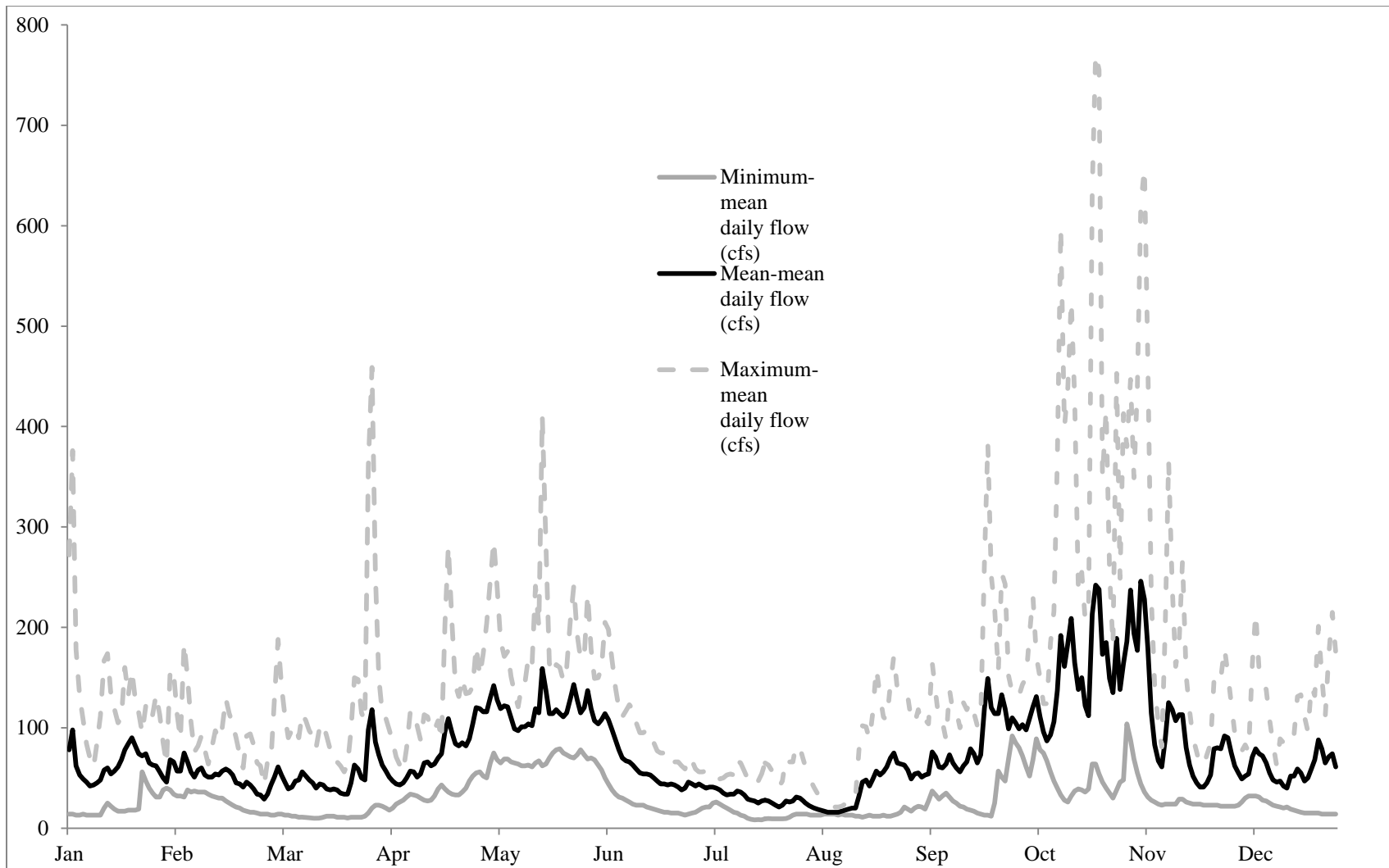
Figure 4.—Annual hydrograph of minimum, mean, and maximum mean daily flows (in cfs) for Sitkoh Creek (October 1, 2006 to September 30, 2011) based on data from streamgage 10303 located at the outlet of Sitkoh Lake.
