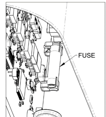
Figure 9: Fuse Replacement view from underside of bowl
