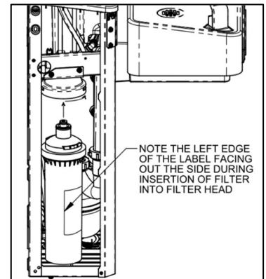
Figure 8: Filter Replacement
