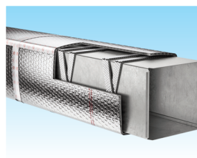
2" Spacer Candy Cane Crisscross
