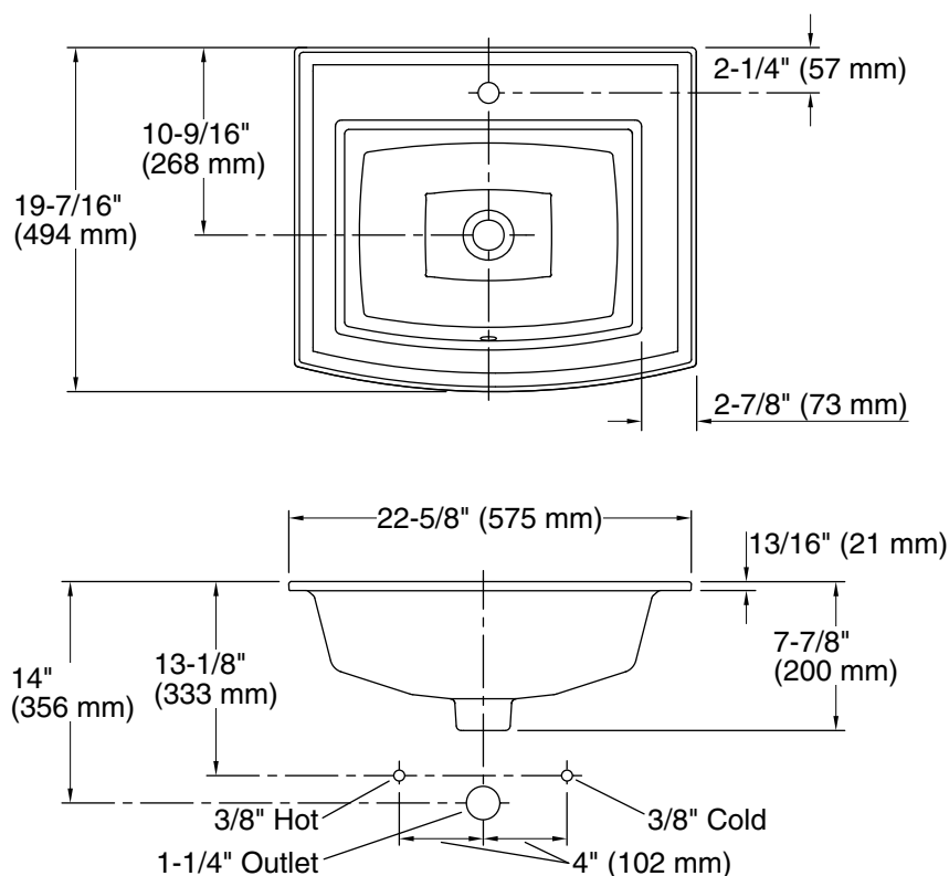
Standard Installation
