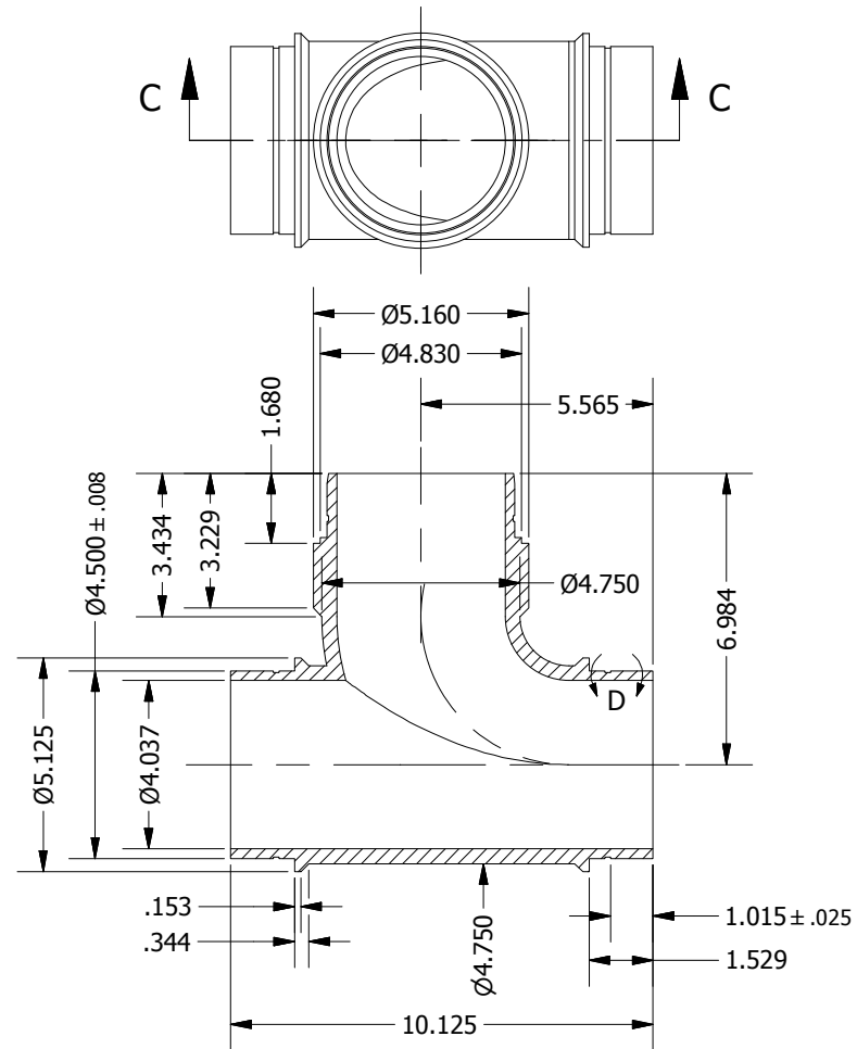
SECTION C-C
