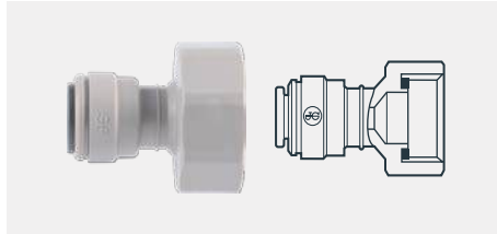
Female Connector BSP Thread
