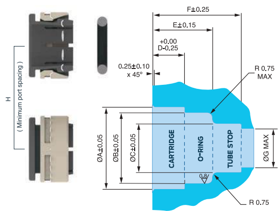
Cavity Dimensional Detail (Metric)
