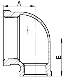
Brass Reducing Elbow
