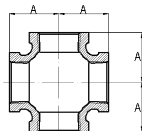
Brass Cross
