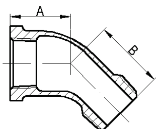
Brass Street Elbow 45
