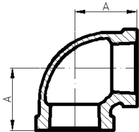
Brass Elbow 90
