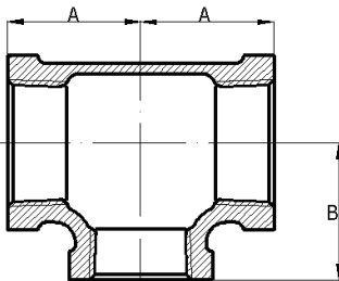
Brass Reducing Tee
