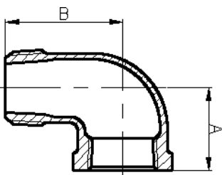
Brass Street Elbow 90
