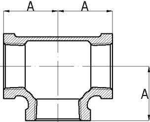
Brass Tee
