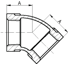
Brass Elbow 45
