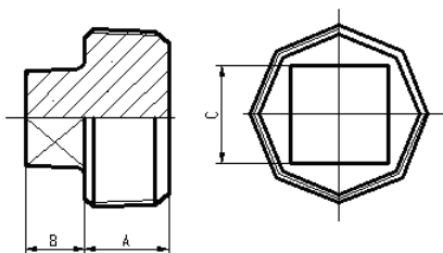
Brass Solid Plug
