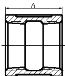
Brass Coupling
