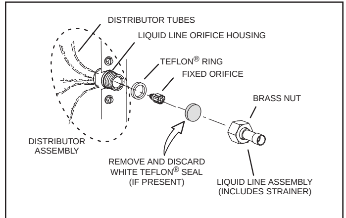
Figure 16. Remove Fixed Orifice (Uncased Coil Shown)
