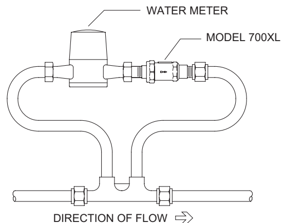
METER SETTER INSTALLATION
