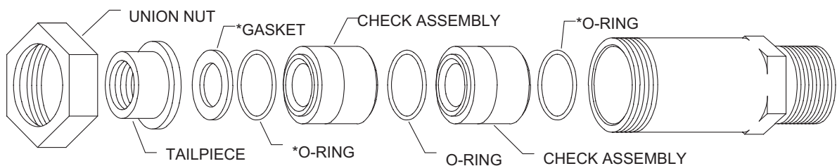
METER SETTER INSTALLATION
