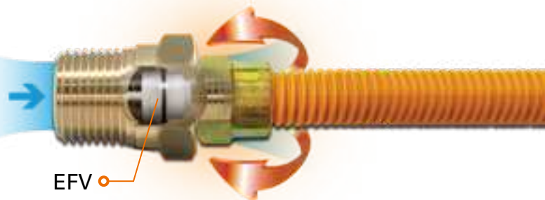
Excess Flow Valve (EFV)
