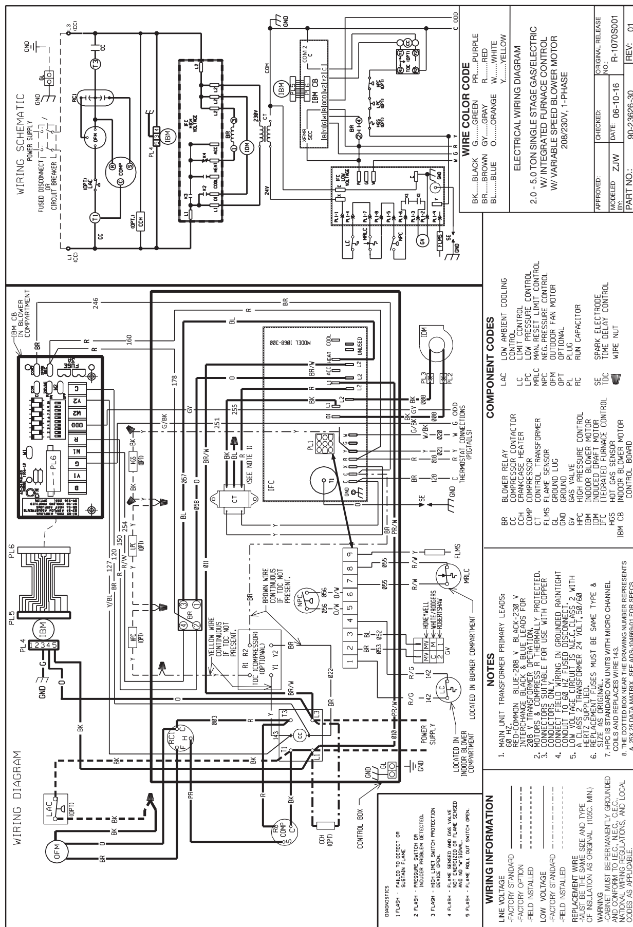
FIGURE 41 WIRING DIAGRAM
