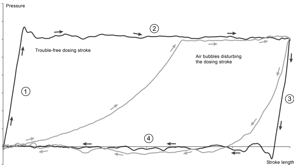
Fig. 17 Indicator diagram
