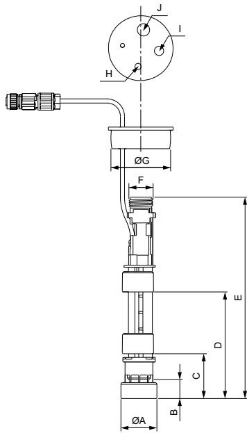
Fig. 33 Flexible level-control unit
