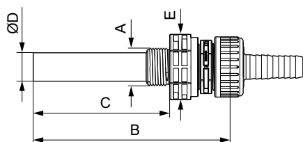
Fig. 34 Injection unit
