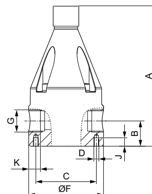
Fig. 42 Pressure loading valve, stainless steel version
