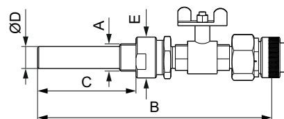
Fig. 36 Injection unit with ball valve, stainless steel version
