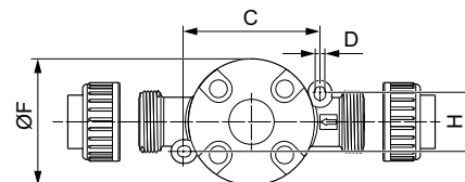
Fig. 41 Pressure loading valve (PP, PVC, PVDF version)
