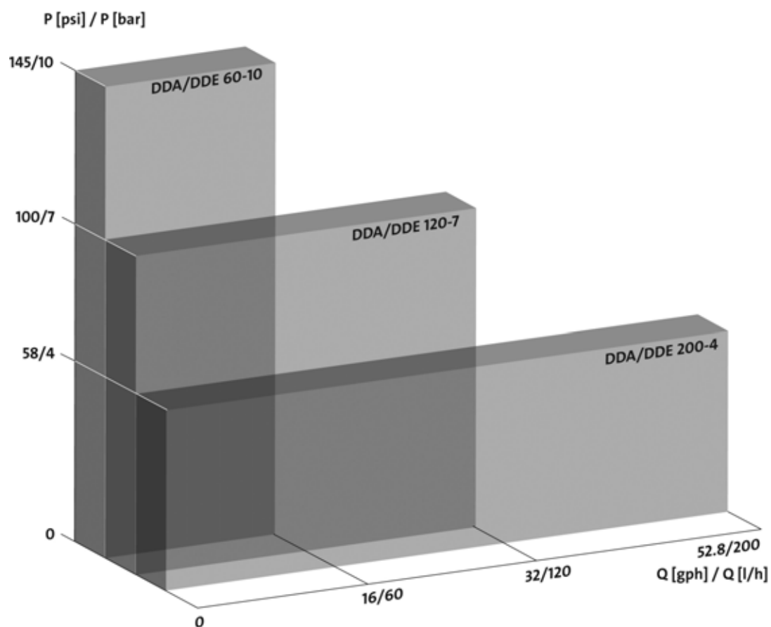
Fig. 1 Performance range
