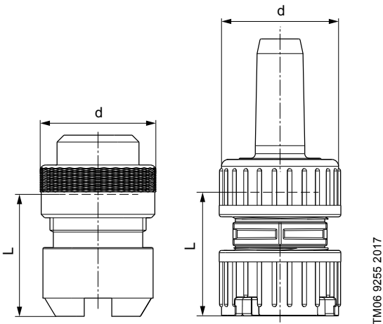
Fig. 27 Foot valves: stainless steel (left), PE/PVDF (right)
