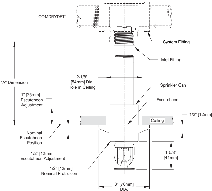
Model F3-56 Dry Pendent Sprinkler: Standard Escutcheon
