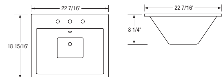
VCS 2219-8WH White (shown) VCS 2219-8BT Biscuit Surface Mount Sink Exterior Dimensions: 22-7/16" x 18-15/16" x 8-1/4"D
