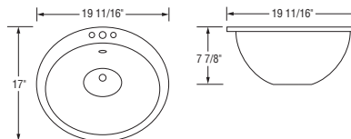
VCS 2017-1WH White VCS 2017-1BT Biscuit VCS 2017-4WH White (shown) VCS 2017-4BT Biscuit VCS 2017-8WH White VCS 2017-8BT Biscuit Surface Mount Sink Exterior Dimensions: 19-11/16" x 17" x 7-7/8"D
