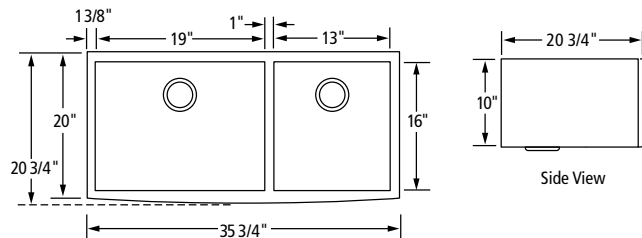
Large Bowl: 19" x 16" x 10"D Small Bowl: 13" x 16" x 10"D Grids not available
