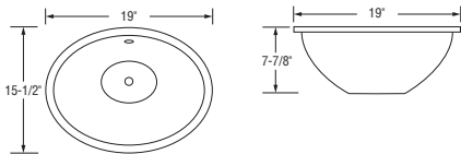
VCS 1915WH White (shown) VCS 1915BT Biscuit Surface Mount Sink Bowl: 19" x 15-1/2" x 7-7/8"D
