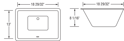
VCU 1913WH White (shown) VCU 1913BT Biscuit Undermount Sink Bowl: 18-29/32" x 13" x 8-1/16"D
