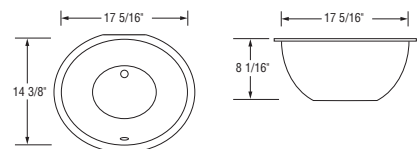
VCU 1714WH White VCU 1714BT Biscuit VCU 1714BK Black (shown) Undermount Sink Bowl: 17-5/16" x 14-3/8" x 8-1/16"D
