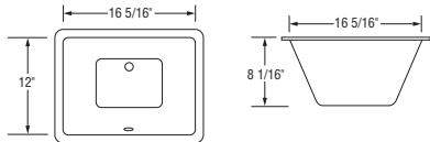
VCU 1612WH White (shown) VCU 1612BT Biscuit Undermount Sink Bowl: 16-5/16" x 12" x 8-1/16"D
