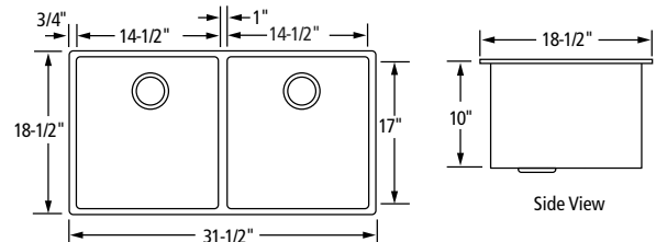
Bowls: 14-1/2" x 17" x 10"D BG-1512S Grid (Optional) 15" x 12"
