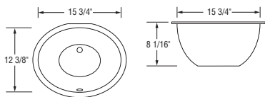
VCU 1512WH White (shown) VCU 1512BT Biscuit Undermount Sink Bowl: 15-3/4" x 12-3/8" x 8-1/16"D
