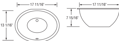
VCU 1713WH White VCU 1713BT Biscuit (shown) Undermount Sink Bowl: 17-11/16" x 13-1/16" x 7-15/16"D
