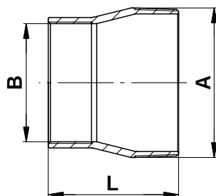
Fig. 26 Dimensional sketch and photo of connecting piece thread-to-thread
