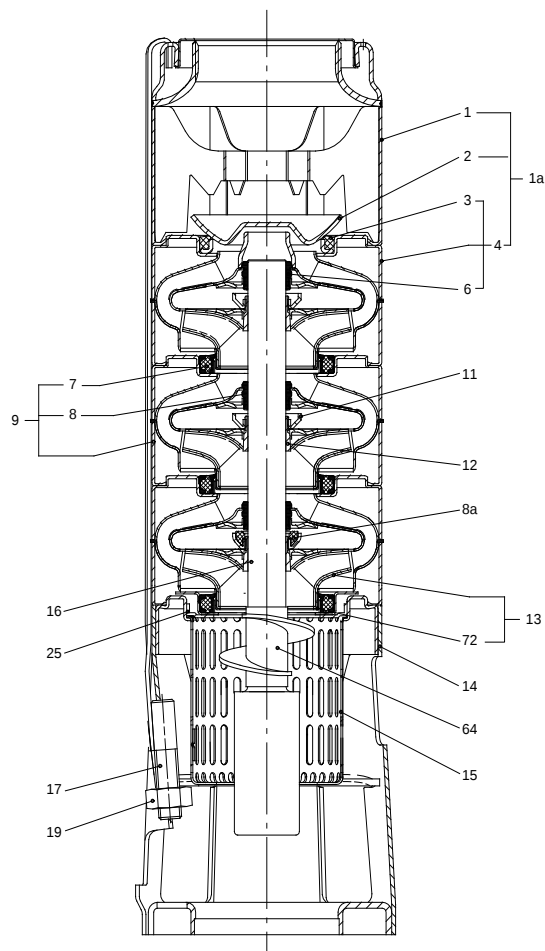
Fig. 14 SP pump, 6"
