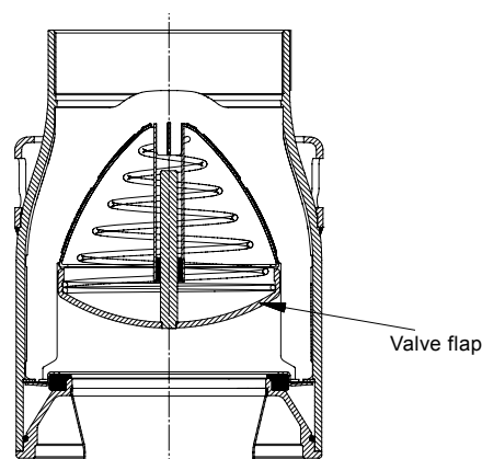
Fig. 5 Check valve
