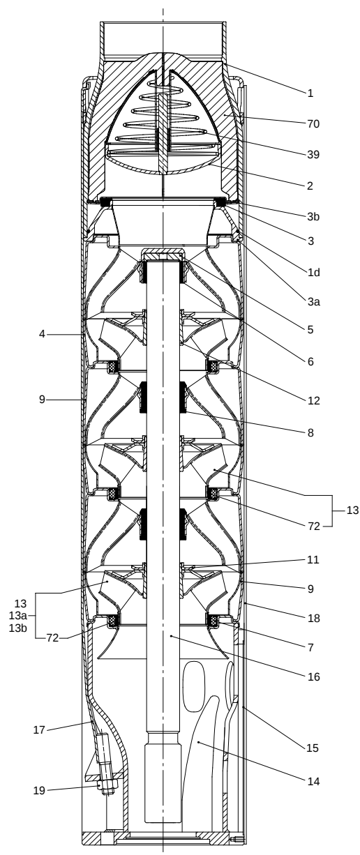
Fig. 16 SP pump, 10"
