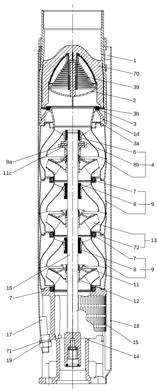
Fig. 15 SP pump, 8"
