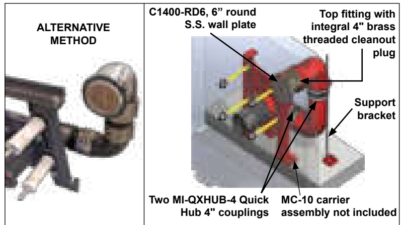
MC-10-CO REAR VIEW
