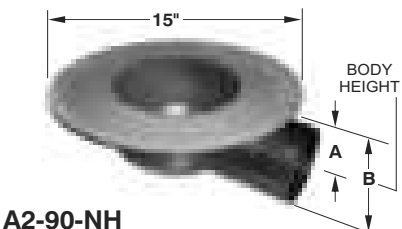
The A2-90-NH No Hub Side Outlet Body
