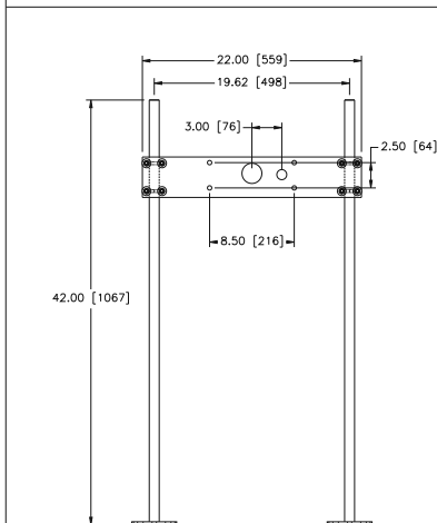
MC-31-HAWS-H1107L CARRIER FOR HAWS H1107L
