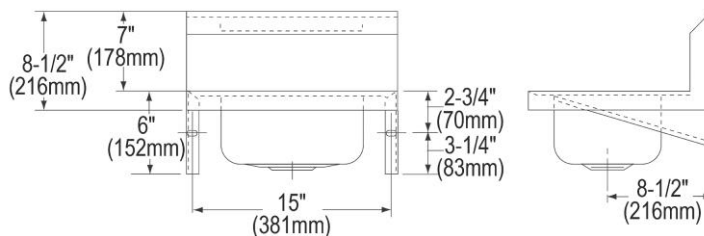
SECTION THROUGH RIM
