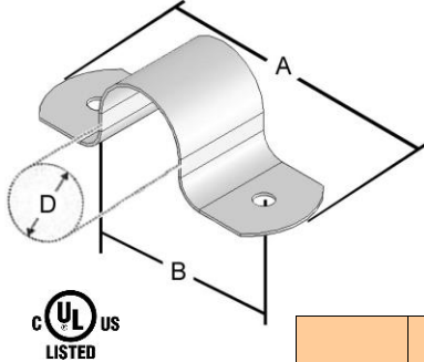
Fig. 070 CPVC TWO-HOLE PIPE STRAP
