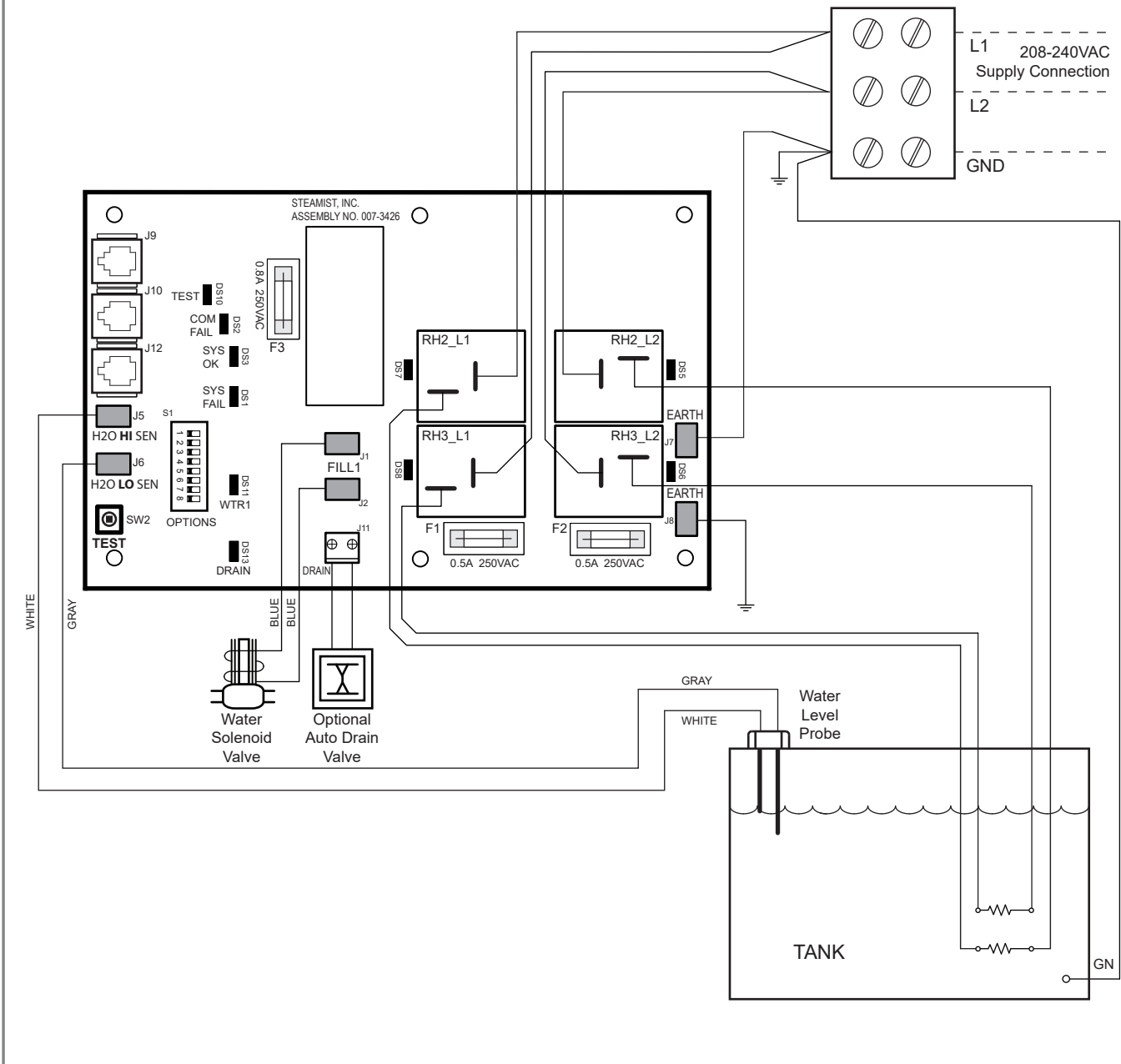
Figure 5 - Wiring Diagram
