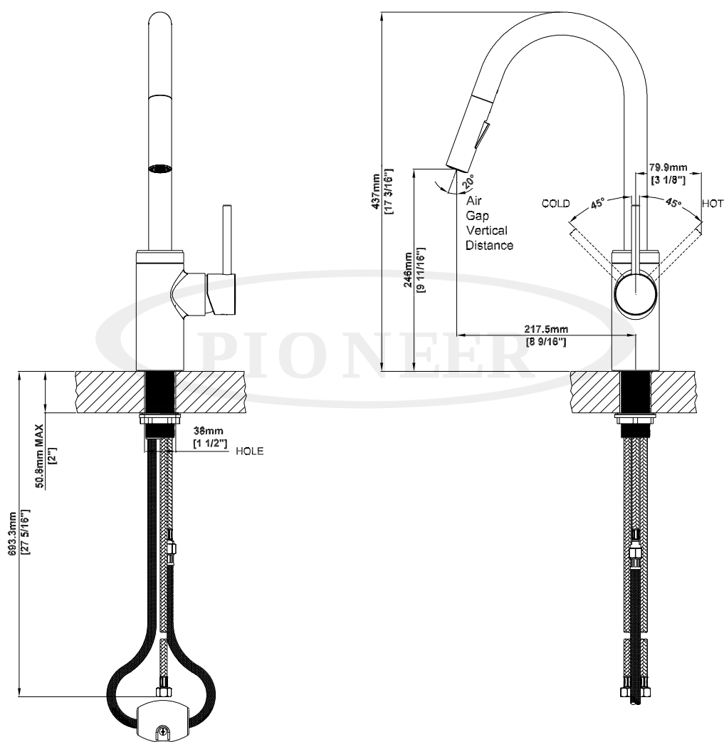
Product Diagram
