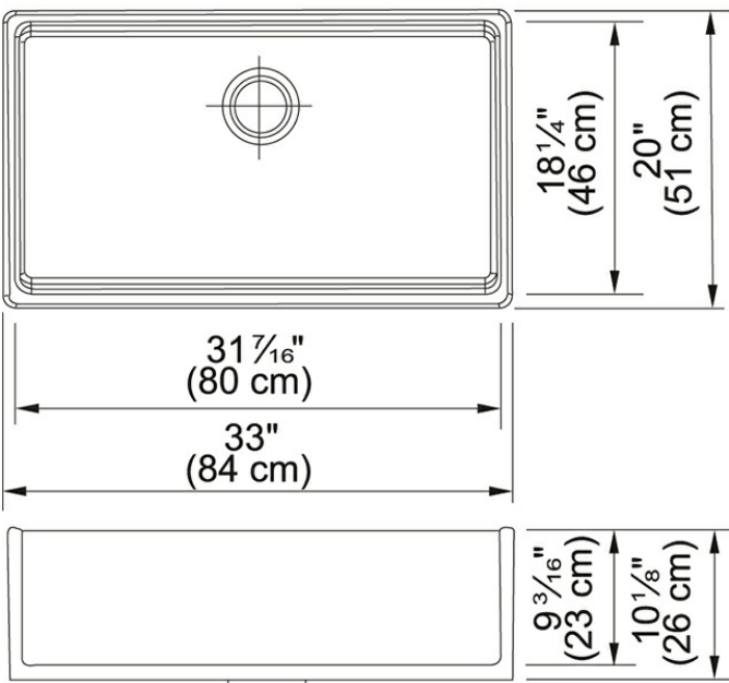
Technical Drawing
