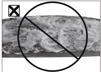
Improperly Lubricated Standard Gasket with Too Much Lubricant
