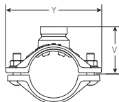
STYLE 922 WITH IGS™ GROOVED OUTLET
