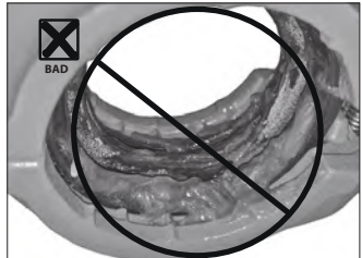
Improperly Lubricated Installation-Ready Gasket with Too Much Lubricant
