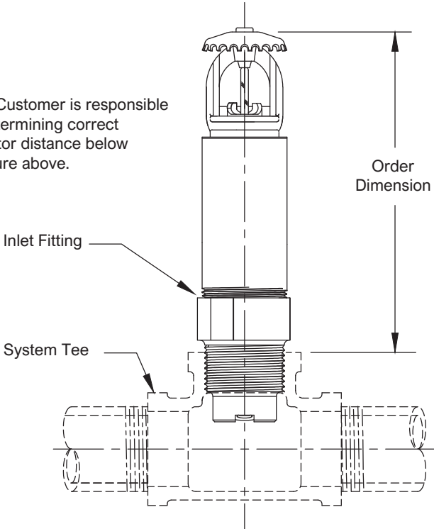
Model F3QR56 Dry Upright Sprinkler
