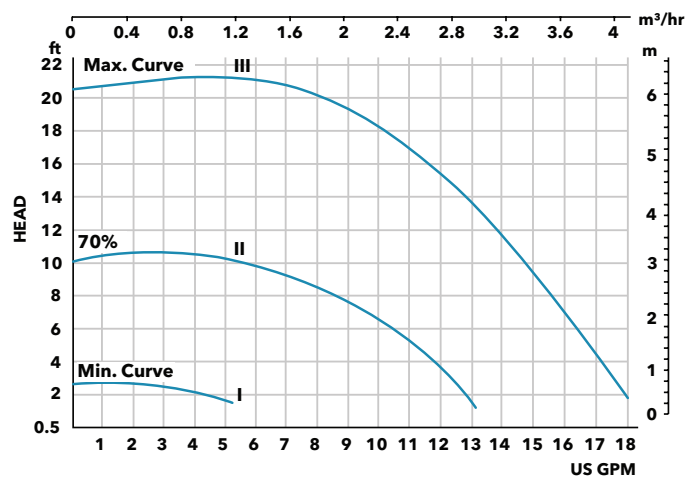
Fixed Speed Curve
