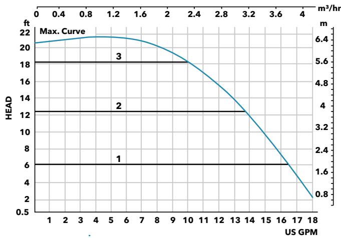
Constant Pressure Curve
