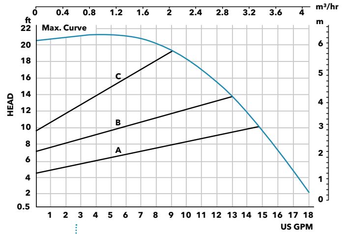
Proportional Pressure Curve
