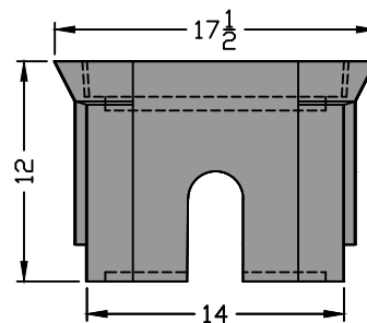
DFW1324C46P-12-4MA<>
