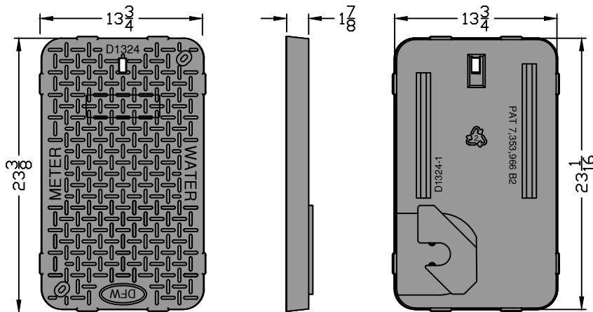
DFW1324C-4MA<>-LID
