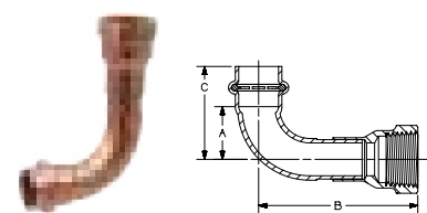
PC607-3 90° Elbow P x F - Wrot
