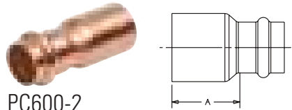
PC600-2 Fitting Reducer Ftg x P – Wrot
