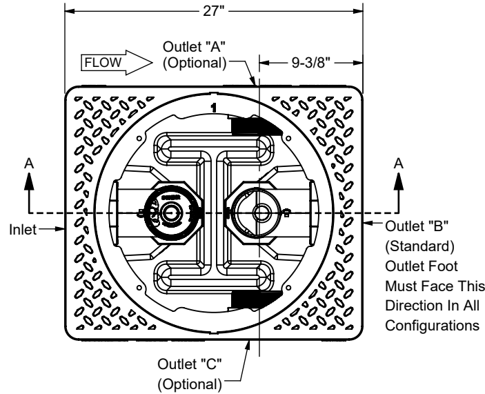
TOP VIEW (COVER REMOVED FOR CLARITY)
