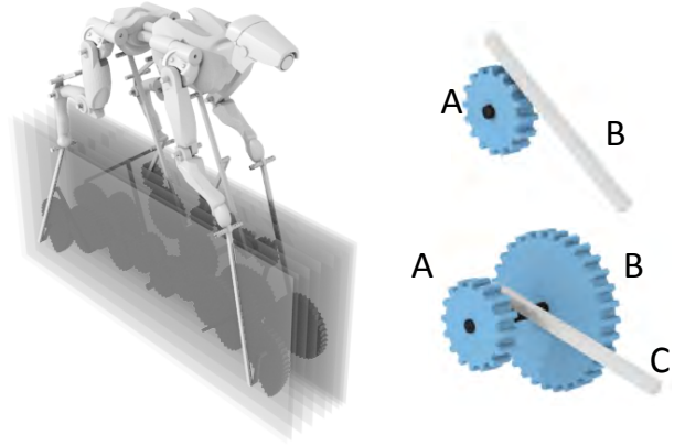
Figure 8: Left: component placement in different planes to remove collisions. Right: types of collisions that can occur between components.
