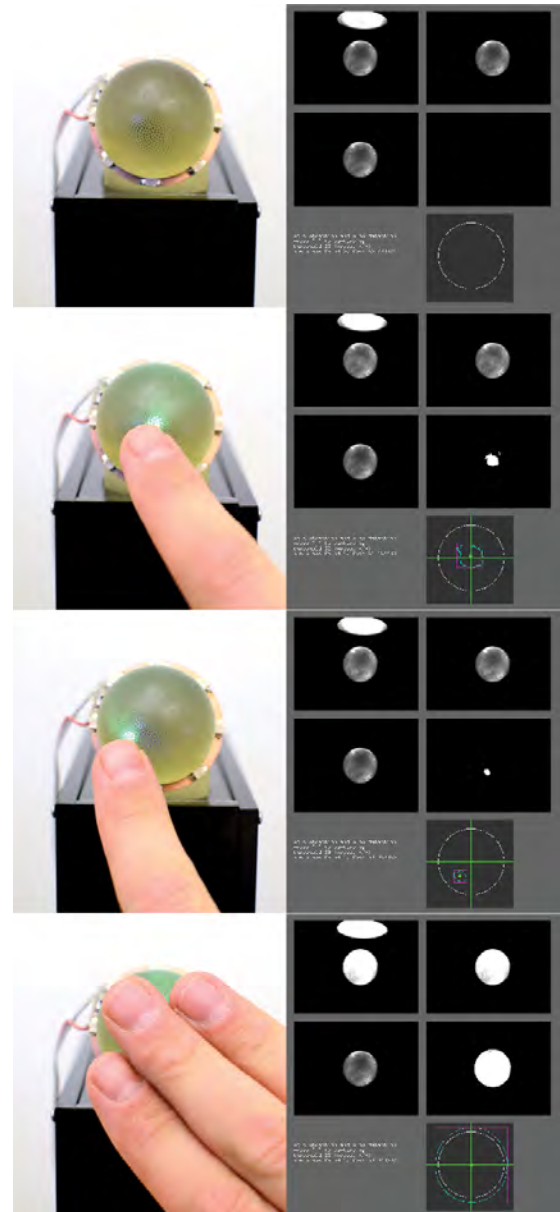
Figure 7. Position sensing on curved display
