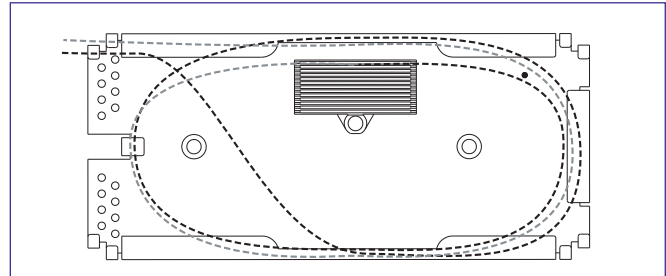
12-Position RTV Splice Closure
