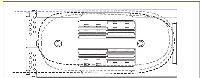
12-Position Mechanical Splice Closure
