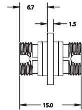
FC Adapter (Regular Flange) | Drawing ZA-2796
