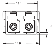
LC Adapter (fits simplex SC footprint) | Drawing ZA-2823
