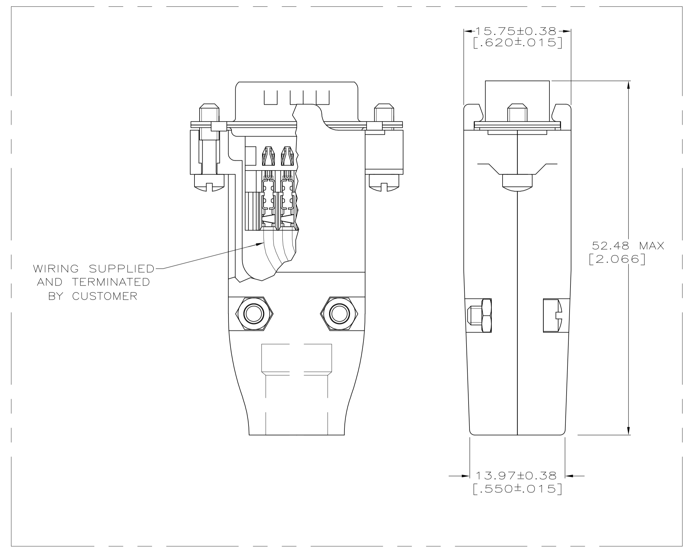
ASSEMBLED VIEW
