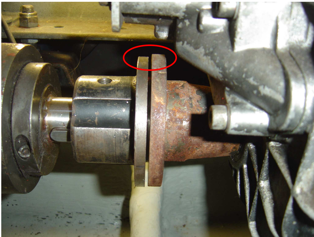
Fixed coupling (left) and gear-box flange off-centered
