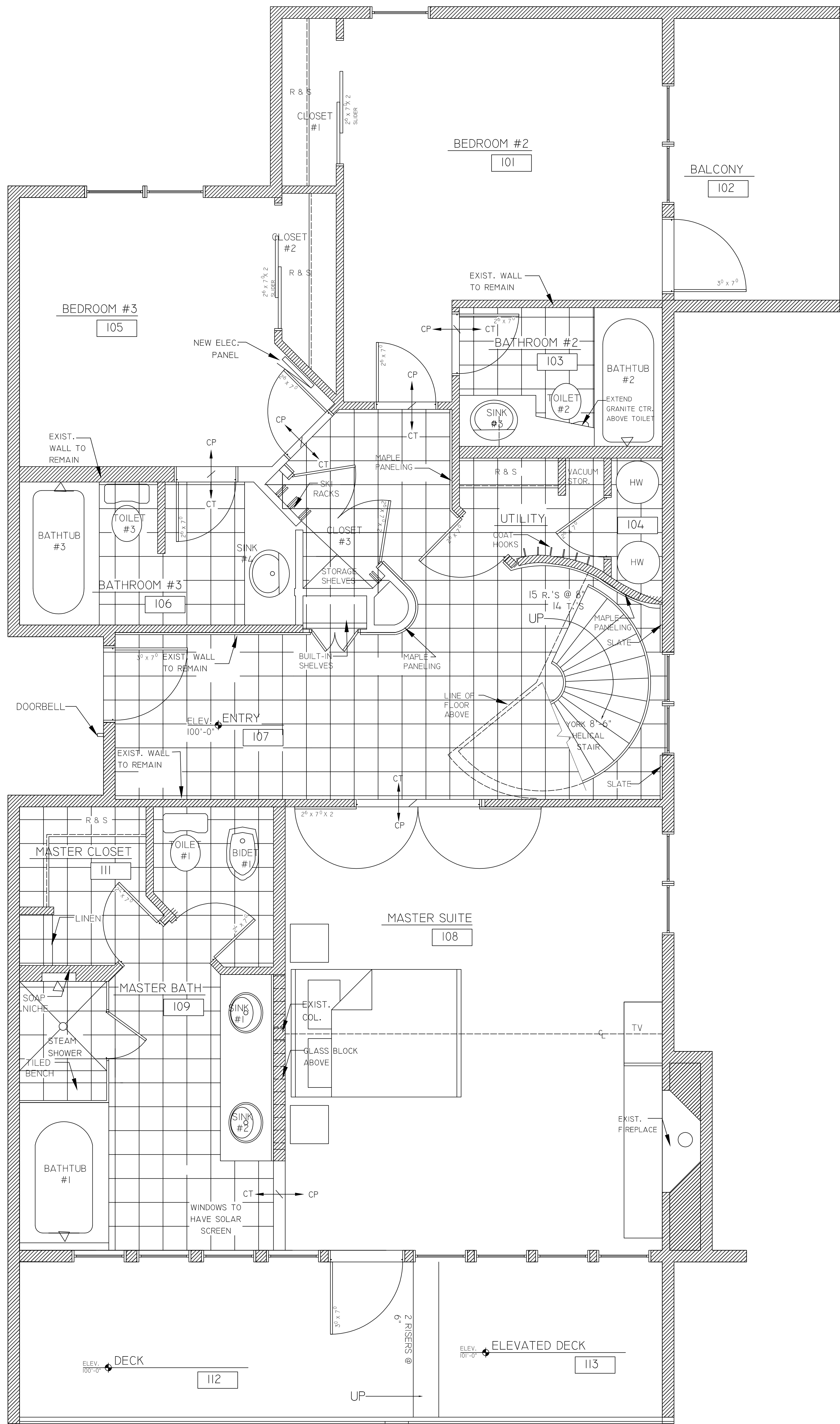
MAIN LEVEL PLAN: FINISHES 1/2" = 1'-0"
