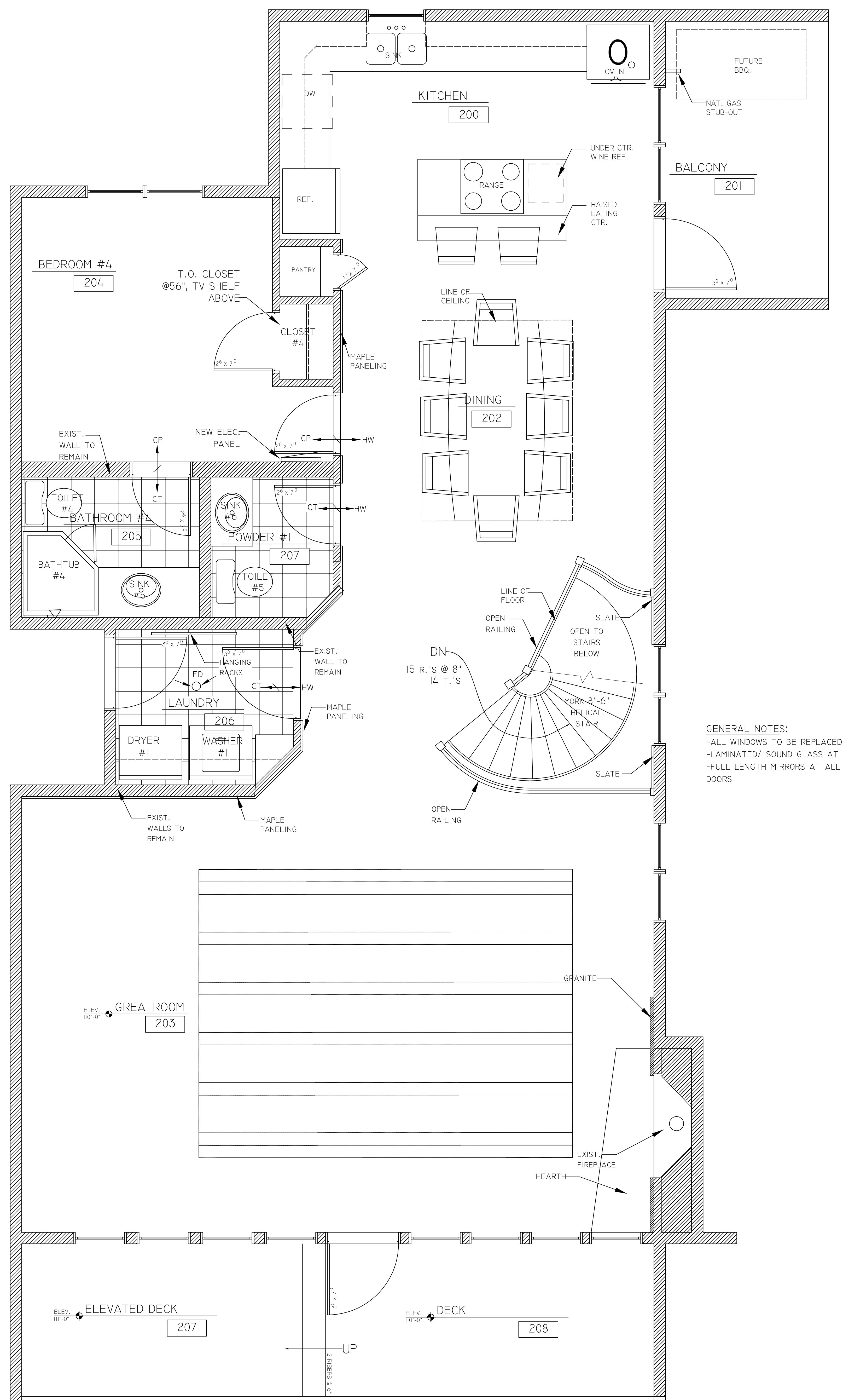
UPPER LEVEL PLAN: FINISHES 1/2" = 1'-0"
