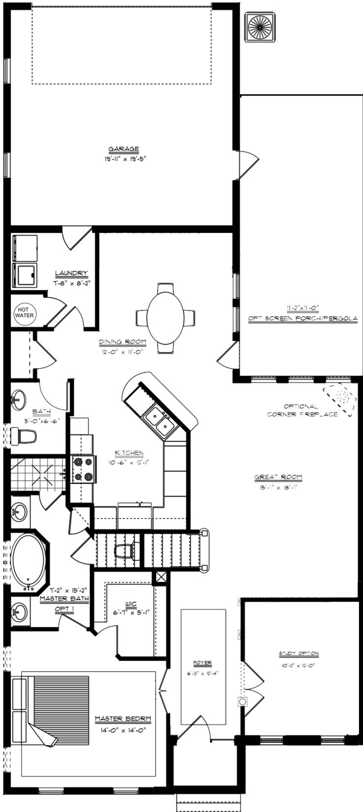
FIRST FLOOR WITH GARAGE
