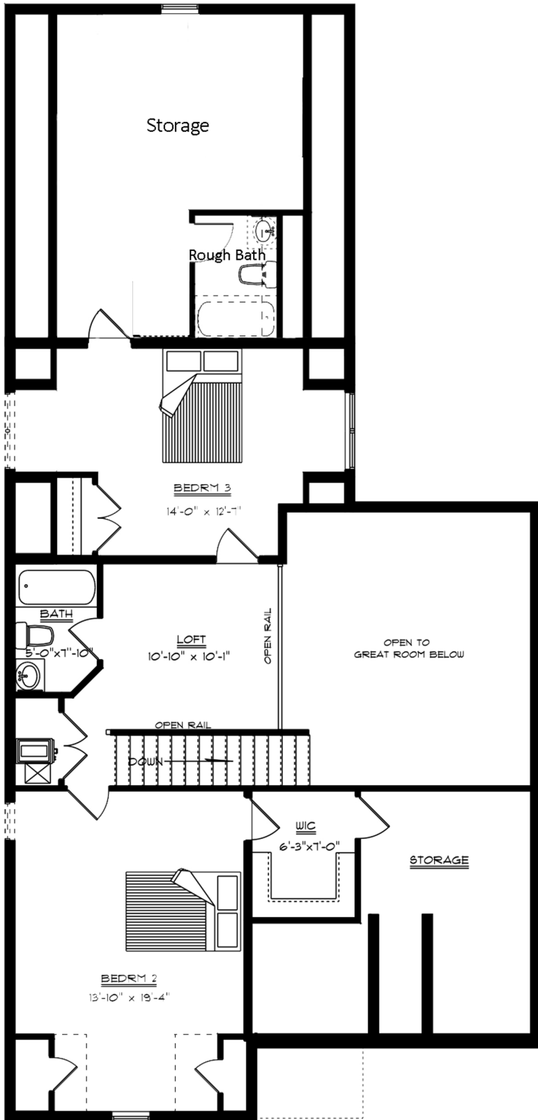
SECOND FLOOR OPTION 1
