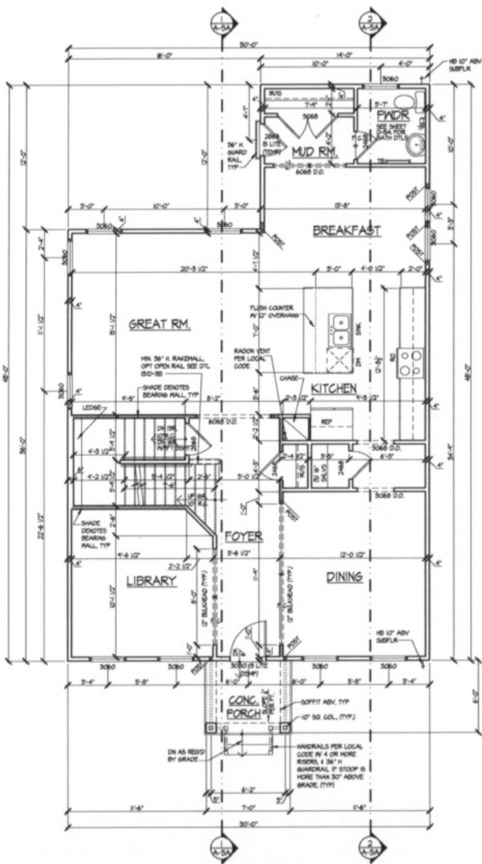
1 MAIN LEVEL PLAN "A" SCALE 1/8"=1'-0"
