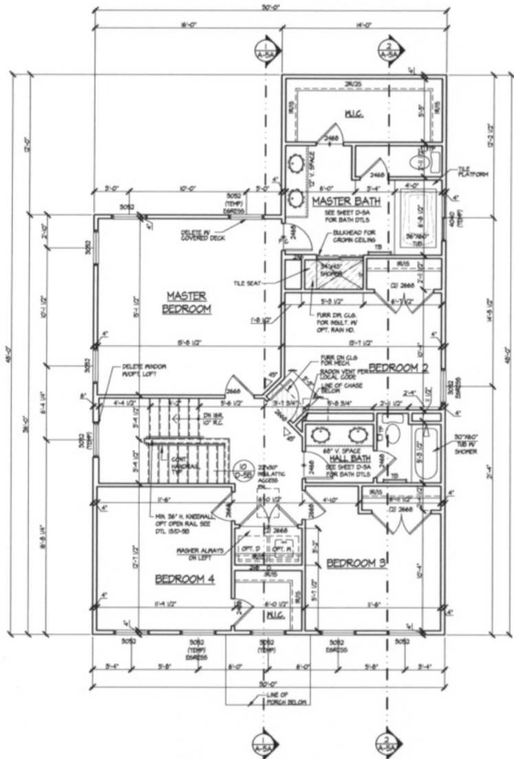
1 UPPER LEVEL PLAN "A" SCALE 1/8"=1'-0"
