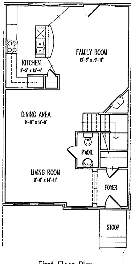
First Floor Plan (24'-0" wide unit)
