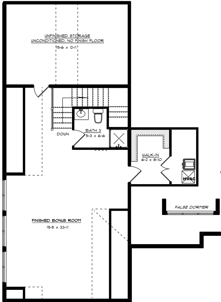
REVERSE OF HOME SHOWN SECOND FLOOR
