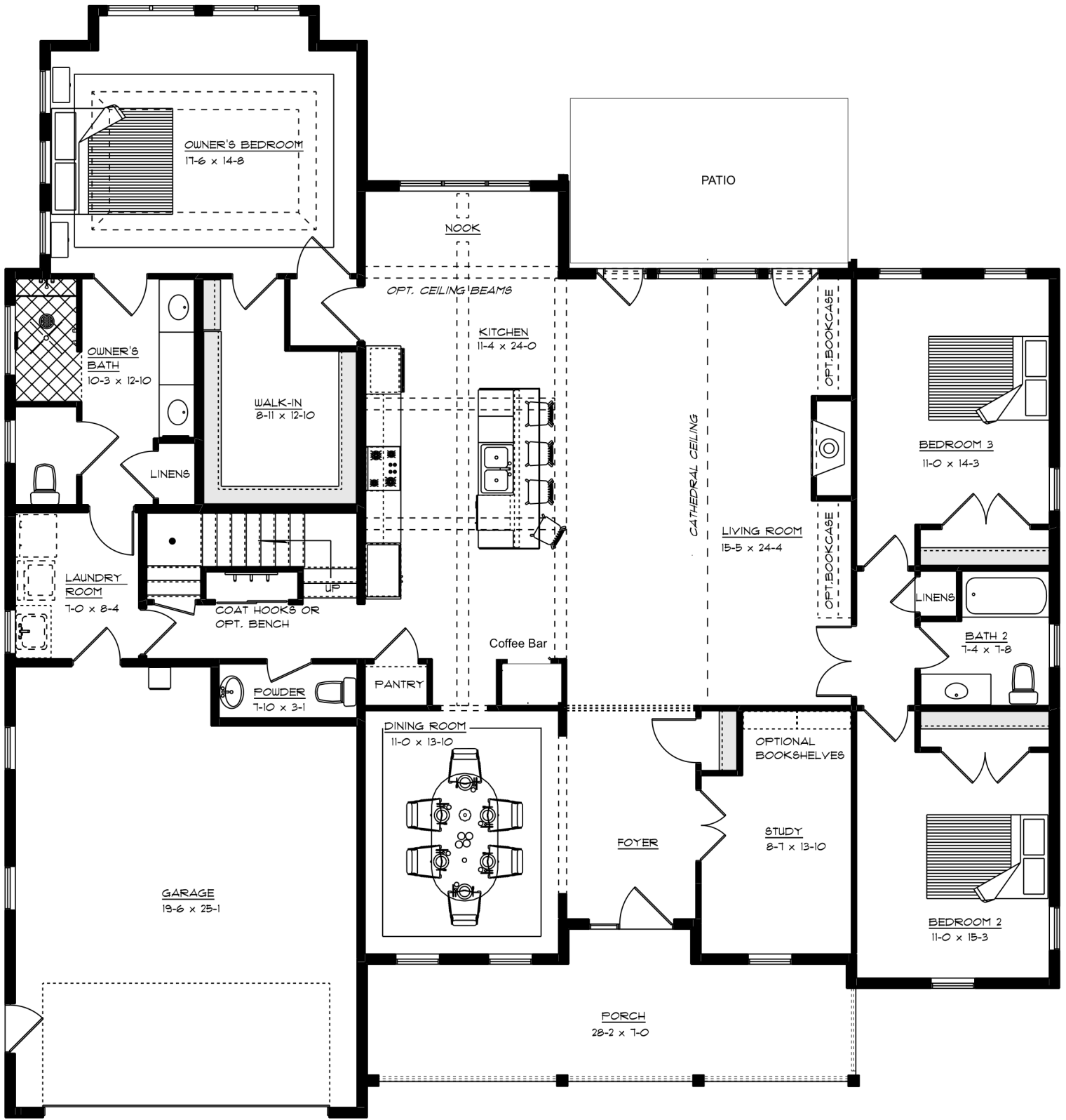
REVERSE OF HOME SHOWN FIRST FLOOR
