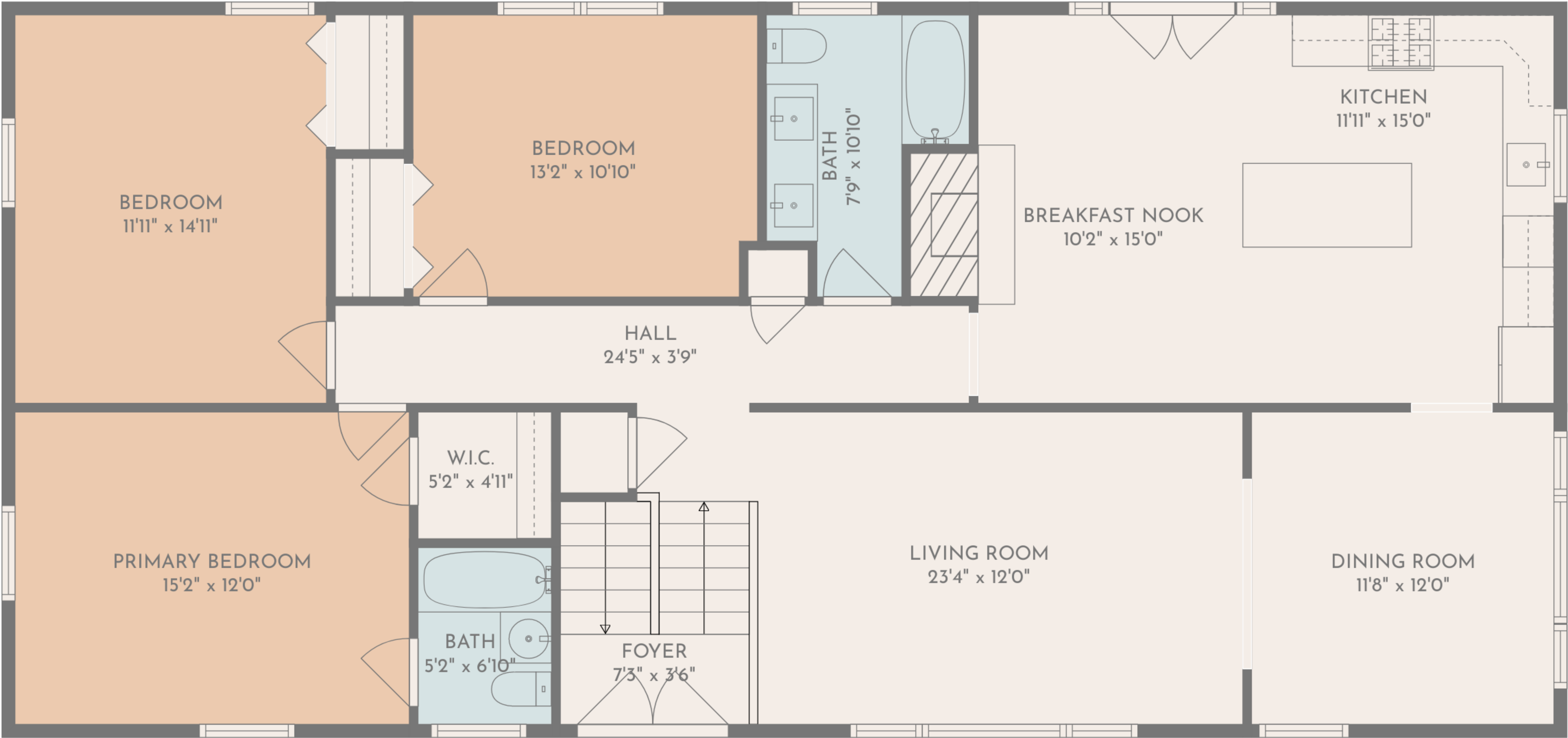
FLOOR 2
