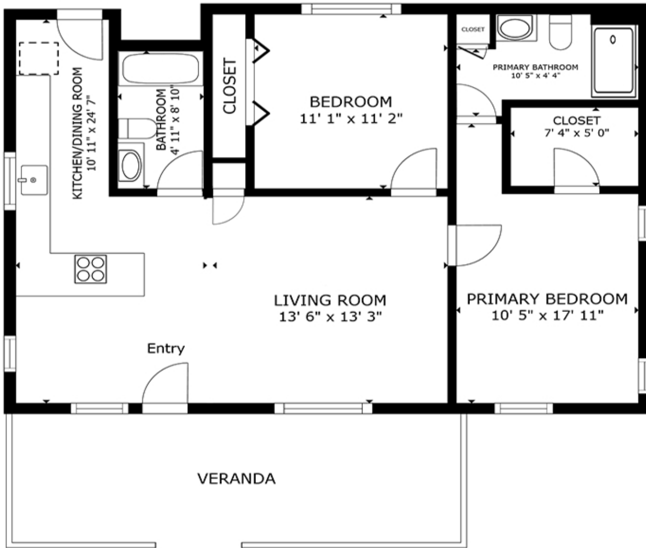
FLOOR PLAN
