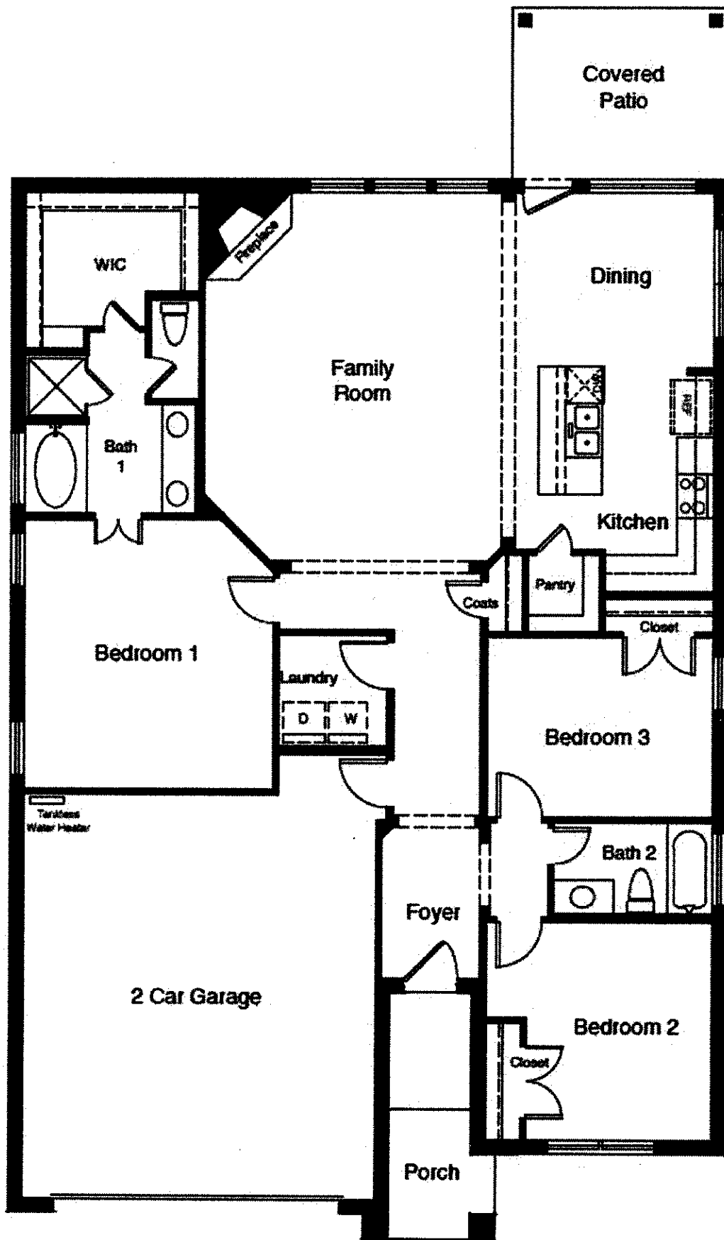
Floor Plan.
