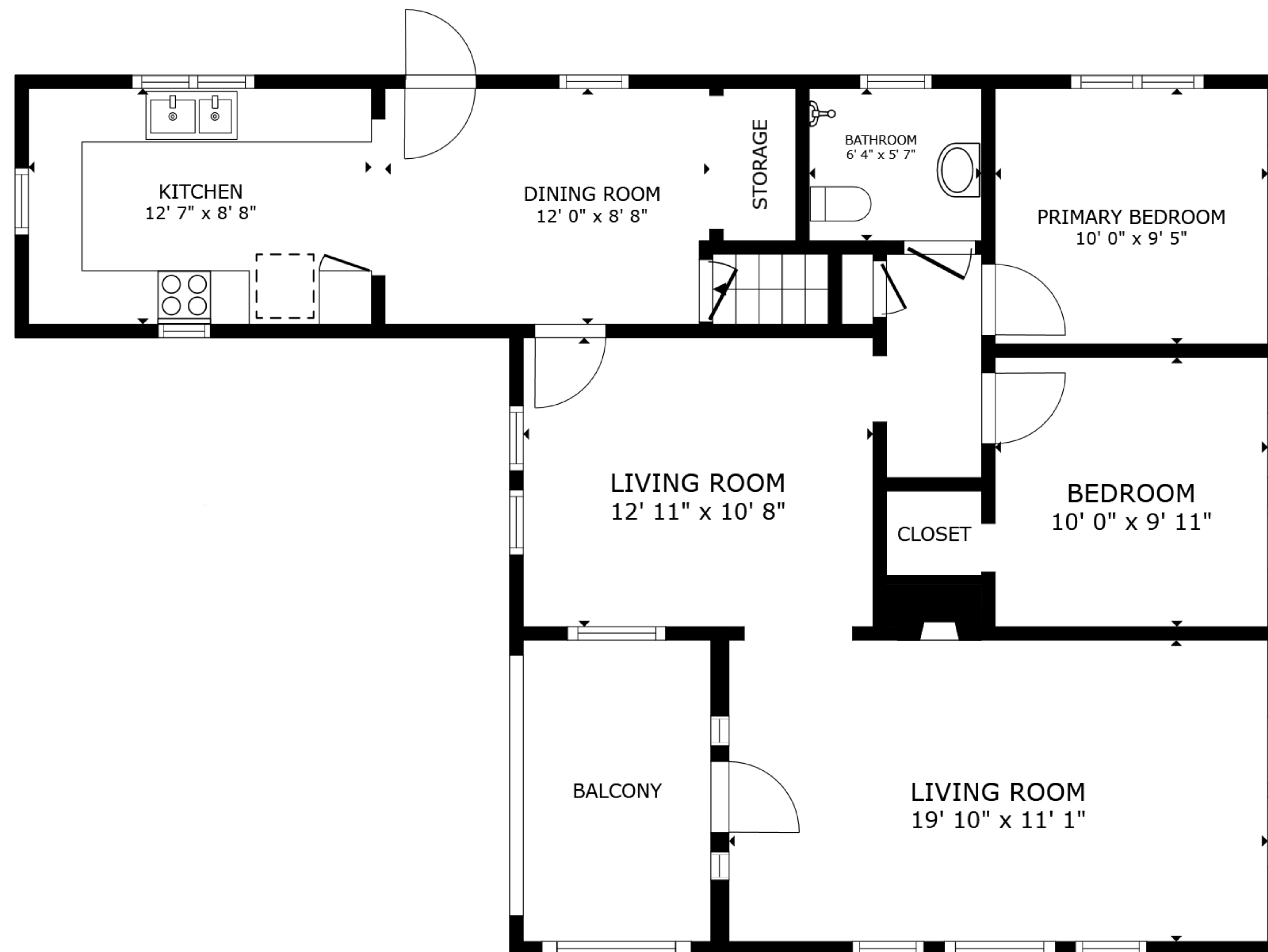
FLOOR 2
