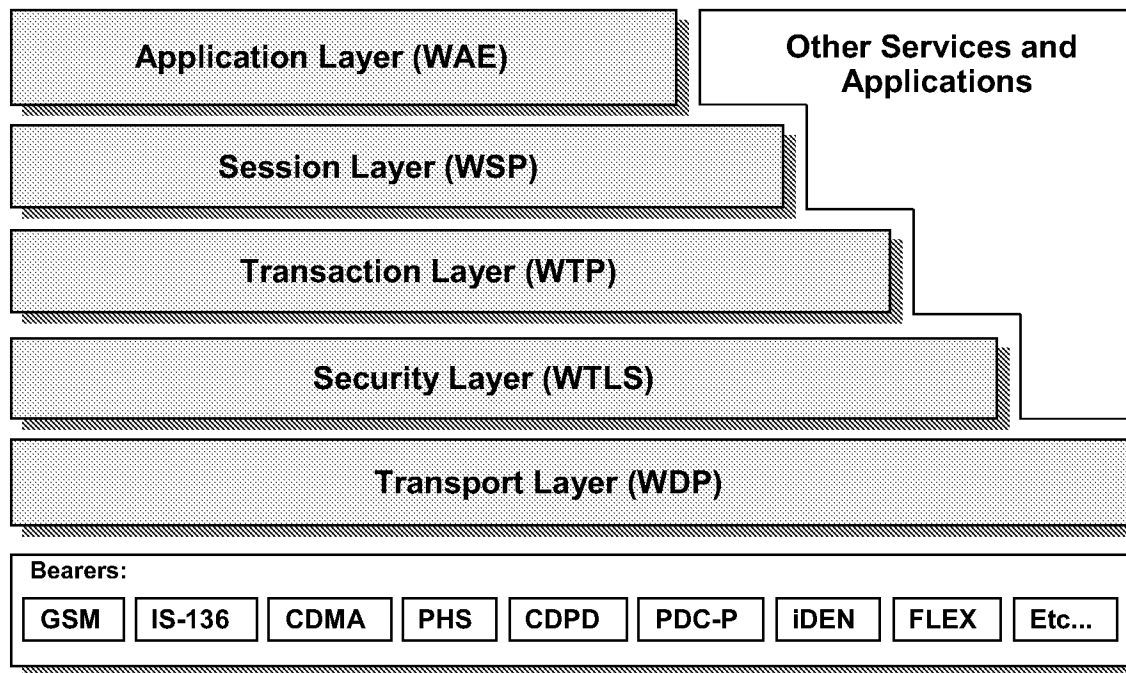
Figure 4. WAP Architecture
