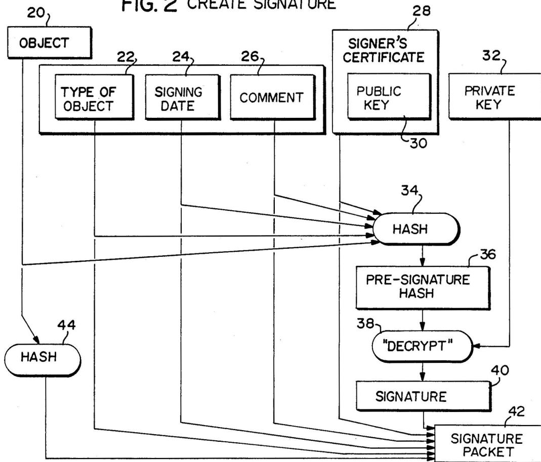
FIG. 2 CREATE SIGNATURE
