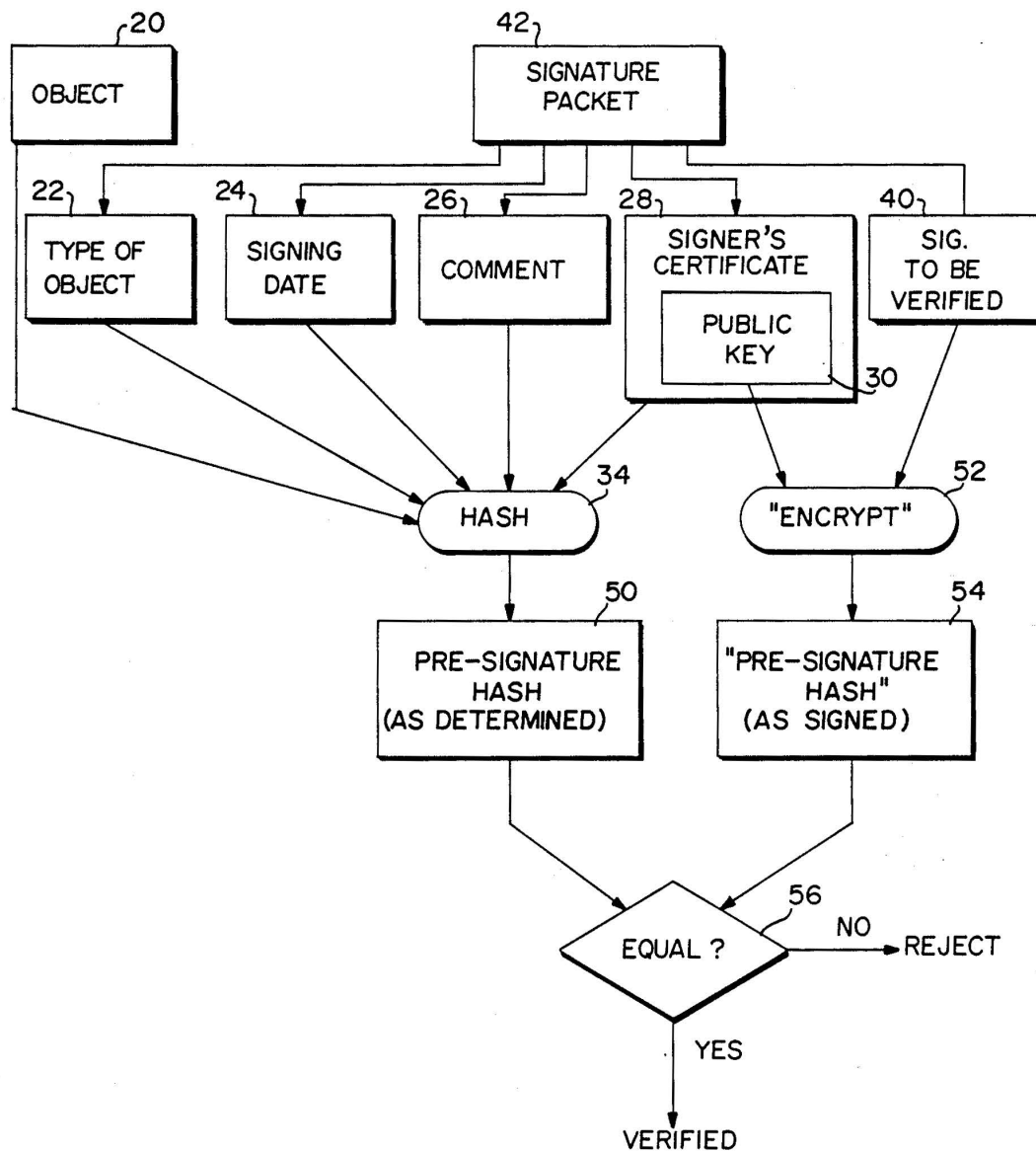
FIG. 3 VERIFY SIGNATURE
