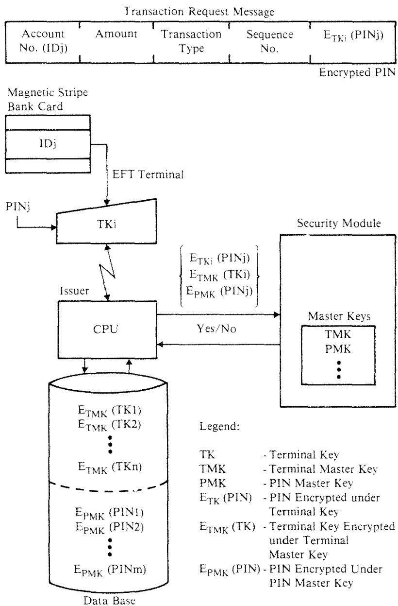
Figure 10-1. Issuer's PIN Validation - Local Transaction
