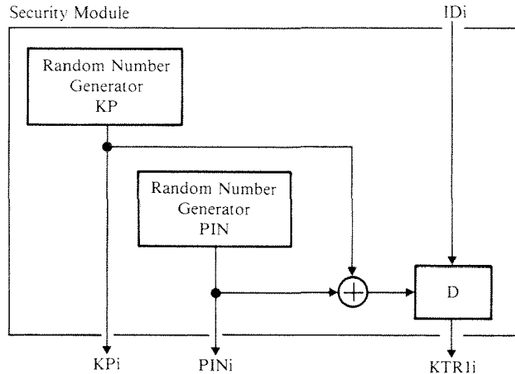
Figure 11-24. Generation of KP, PIN, and KTR1 in Issuer's Security Module - Initialization Process
