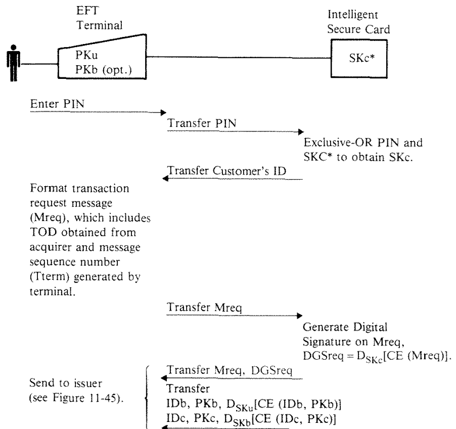
Figure 11-44. On-Line Use—EFT Terminal
