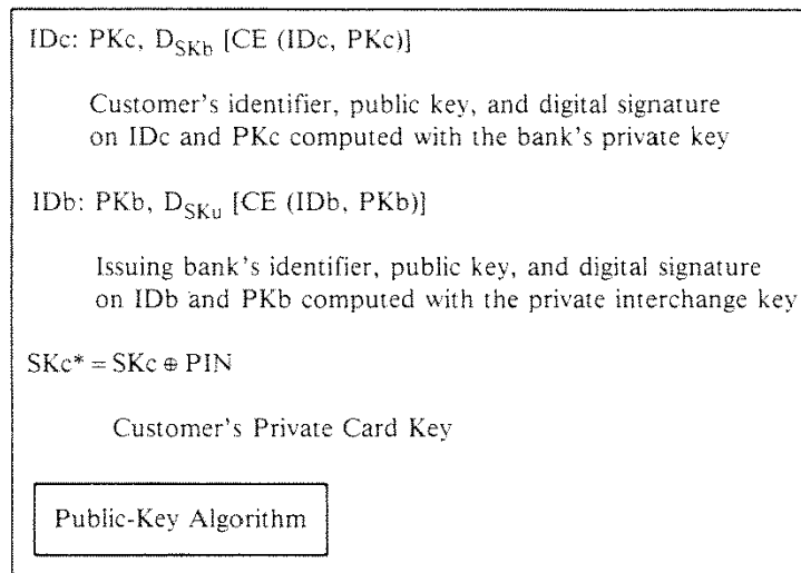
Figure 11-41. Information Stored on the Intelligent Secure Card
