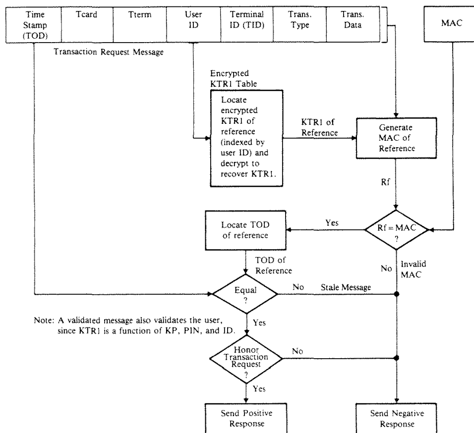
Figure 11-28. Message Authentication at the Issuer's EDP System
