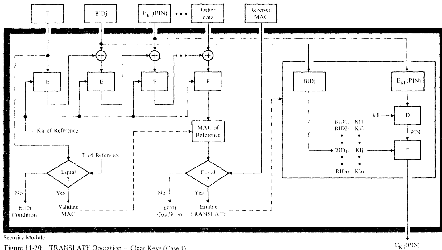
Figure 11-20. TRANSLATE Operation — Clear Keys (Case 1)
