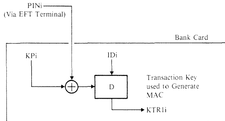
Figure 11-25. Regeneration of the Transaction Key on the Bank Card - Part of the Verification Process
