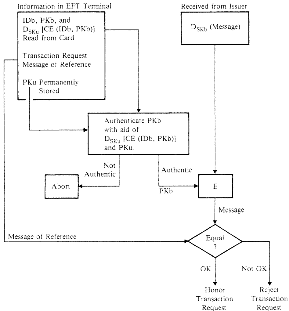
Figure 11-46. On-Line Use—EFT Terminal
