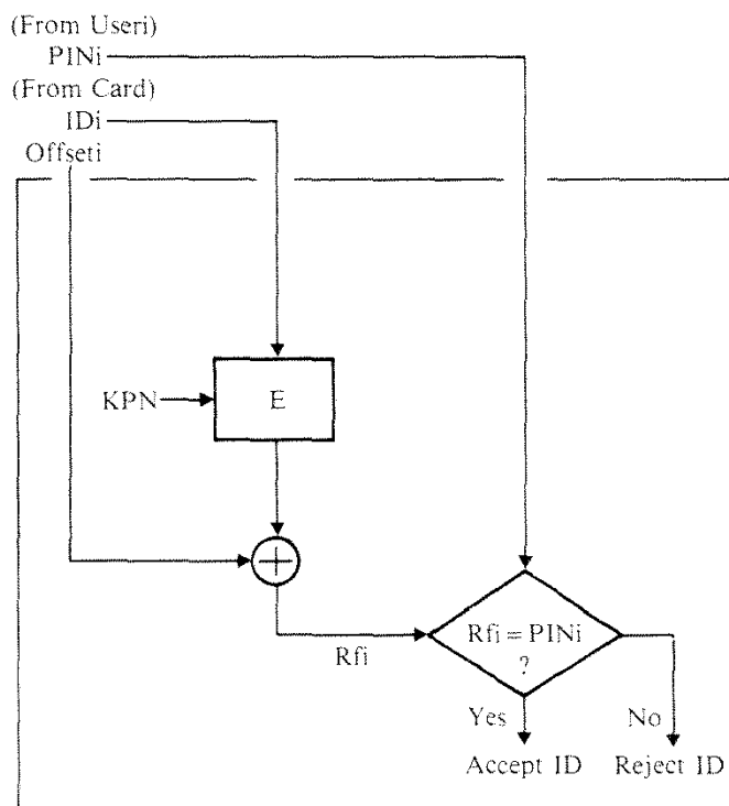
Figure 11-13. An Example of Off-Line Personal Verification with User-Generated PINs Employing an Offset
