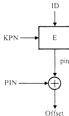
Figure 11-7. Personal Verification Using a PIN Offset
