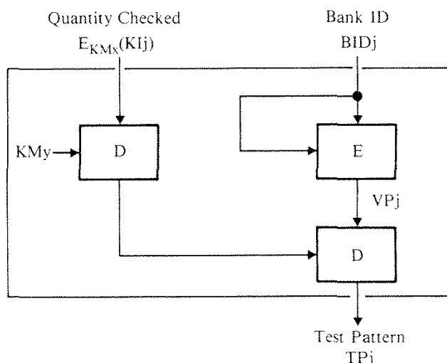
Figure 11-21. Generation of Test Pattern
