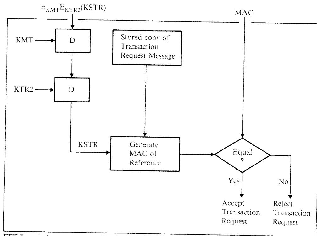
Figure 11-30. Message Authentication at the EFT Terminal
