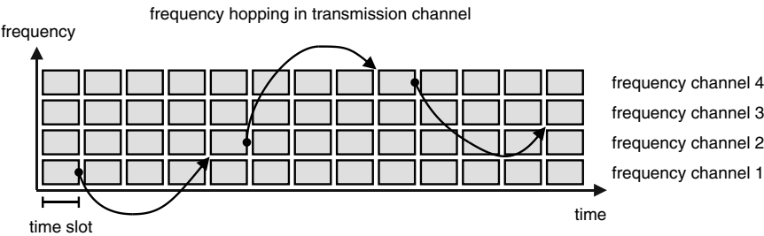
Figure 13.3 Frequency–time diagram for time-division multiple access (TDMA) with frequency hopping. Here each frequency channel is allocated four transmission channels. Each of the gray rectangles represents one signal burst. The regions between the frequency channels and time slots are guard bands and guard times for suppressing interference between the individual signal bursts
