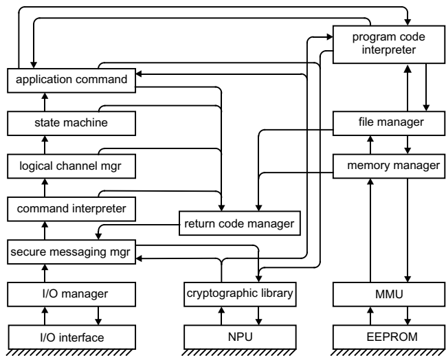
Figure 5.2 Command processing within a smart card operating system. The level of hardware abstraction increases from the bottom to the top in this figure. The program code interpreter is optional
