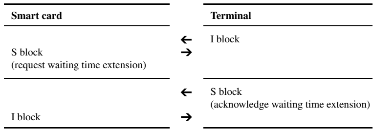
Figure 6.36 Procedure for extending the waiting time
