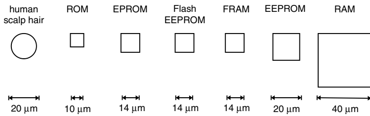
Figure 3.47 Comparison of the die area of a single bit cell for various types of memory. The dimensions shown here are approximate and relate to 0.8-μm technology. For comparison, the diameter of the first planar transistor in 1959 was 764 μm [Buchmann 96, Stix 96], the diameter of the dot at the end of each sentence in this book is 400 μm, the resolution limit of the human eye is 40 μm, the size of a bacterium is 0.4–2 μm and the size of a DNA double helix is 0.1 μm
