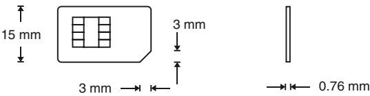
Figure 3.3 The ID-000 format. Thickness: 0.76 mm ± 0.08 mm; corner radius: 1 mm ± 0.10 mm; corner: 3 mm ± 0.03 mm. The dimensions shown indicate the size of the card excluding tolerances
