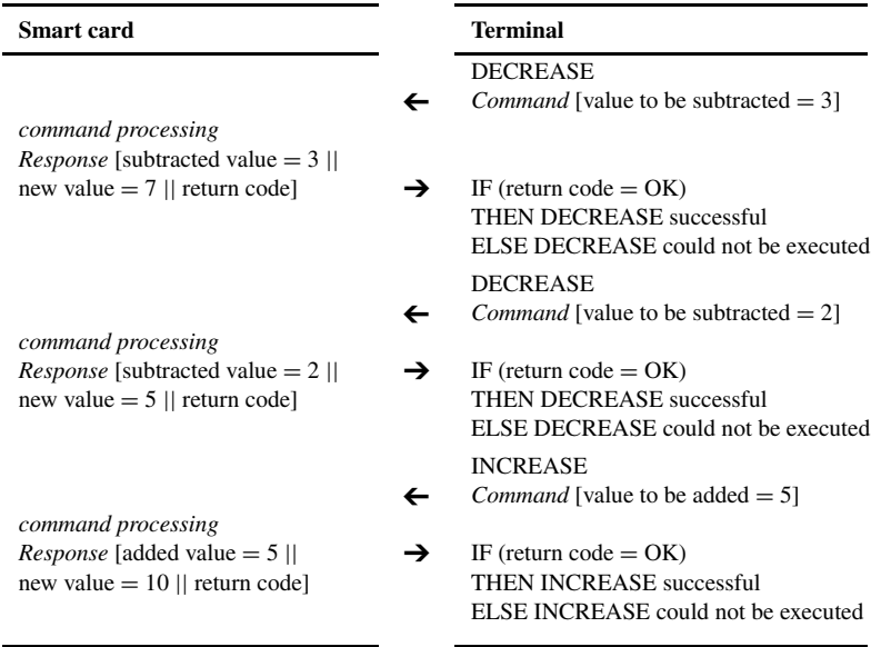
Figure 7.12 Sample command sequence using INCREASE and DECREASE
