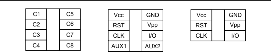
Figure 3.34 Electrical assignments and numbering of smart card contacts, per ISO 7816-2
