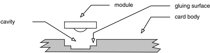
Figure 3.23 Inserting the chip module in a milled opening in the card body
