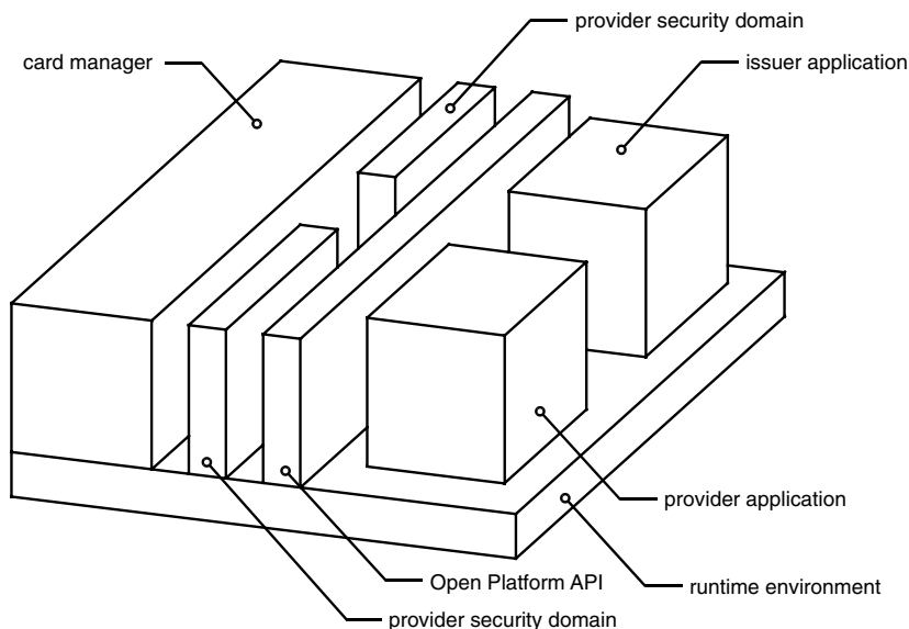
Figure 5.38 Basic architecture and components of Open Platform
