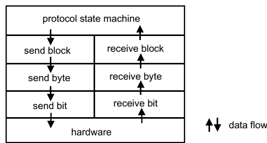
Figure 5.3 The portion of the command processing sequence performed within the I/O manager of a smart card operating system
