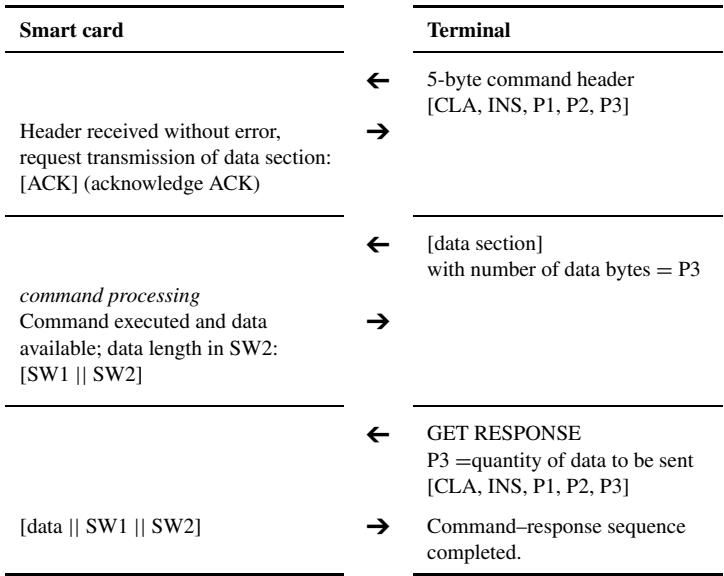
Figure 6.28 A typical T = 0 communications sequence with data in both the command and the response (a Case 4 command, such as MUTUAL AUTHENTICATE)
