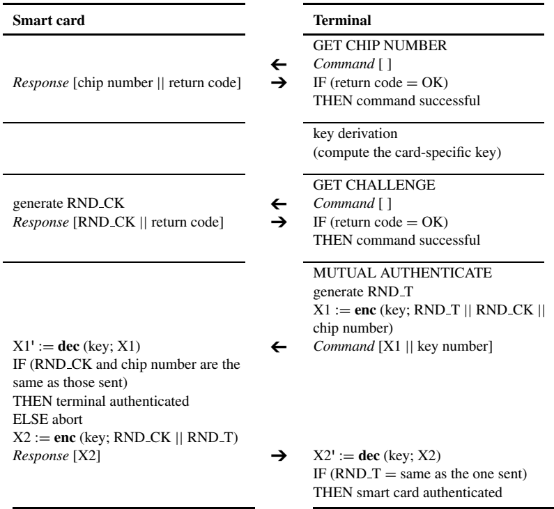
Figure 7.15 Sample command sequence using MUTUAL AUTHENTICATE
