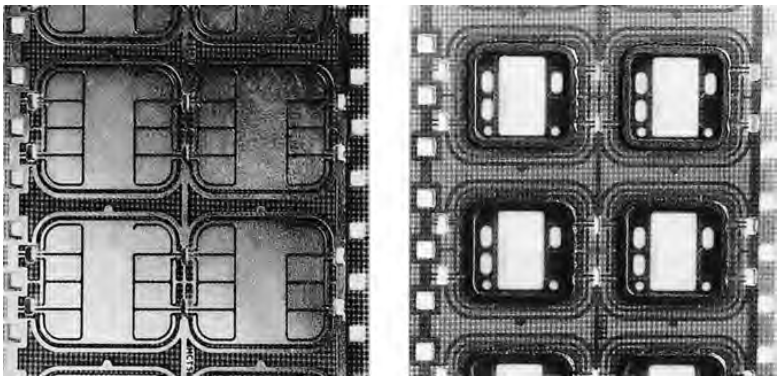
Figure 3.24 Front and rear views of chip-on-flex modules on 35-mm tape. The five openings in the carrier circuit board, for the bonding wires that make the electrical connections to the chip, can be clearly seen in the rear view
