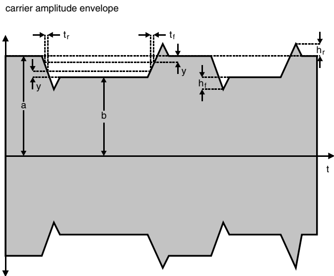
Figure 3.90 Type-B carrier modulation. A continuous supply of energy is made possible by the small modulation index (10 %). Here t_r, t_f \leq 2\text{ }\mu\text{s} , y = 0.1 \cdot (a - b) and h_r, h_f \leq 0.1 \cdot (a - b)
