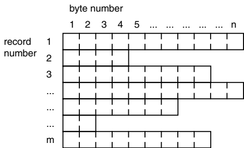
Figure 5.23 Linear variable file structure
