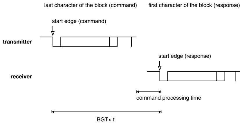
Figure 6.35 Definition of the block guard time (BGT)
