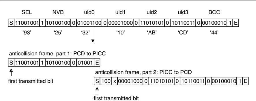
Figure 3.99 Two examples of bit-oriented anticollision frames. In the first example, the frame is divided after a full byte, while in the second example it is divided after the fifth bit of a data byte
