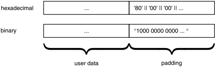
Figure 4.33 Data padding according to ISO/IEC 9797, Method 2
