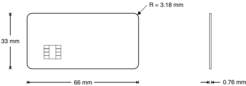
Figure 3.4 The ID-00 format. Thickness: 0.76 mm ± 0.08 mm; corner radius: 3.18 mm ± 0.30 mm. The dimensions shown indicate the size of the card excluding tolerances
