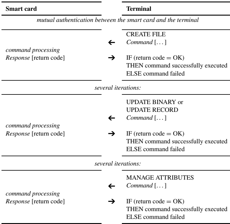
Figure 7.18 Sample procedure for loading a new application
