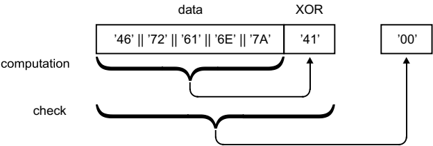
Figure 4.13 Computing and checking an XOR checksum
