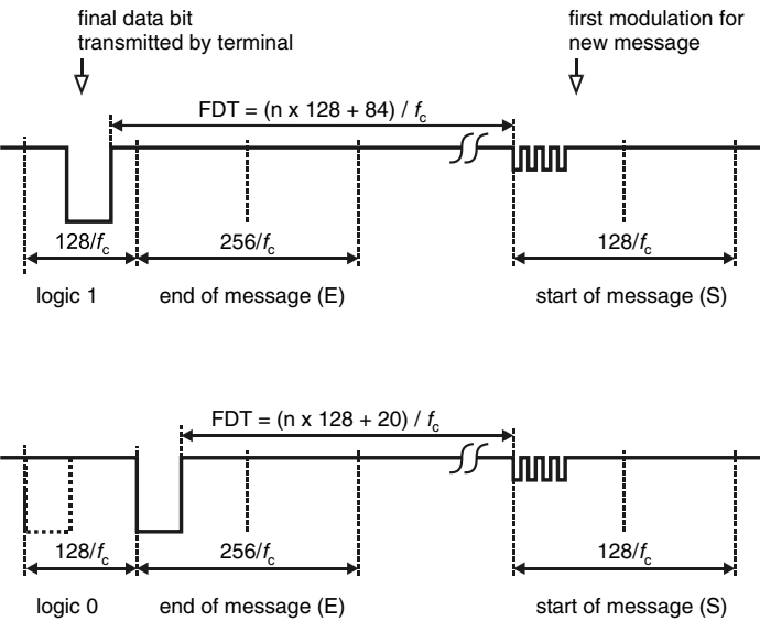
Figure 3.98 Frame delay time PCD to PICC (FDT)
