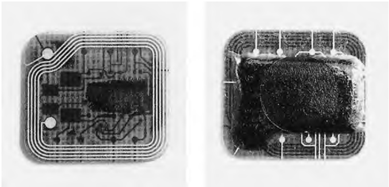
Figure 10.35 Front and rear views of a module with an integrated coil for a microcontroller chip
