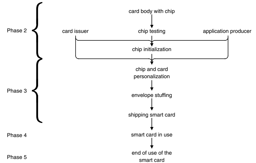
Figure 10.51 Phases 2 through 5 of the smart card life cycle: testing, initialization, personalizing, use and end of use
