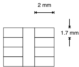
Figure 3.66 Minimum contact dimensions as specified in ISO 7816-2
