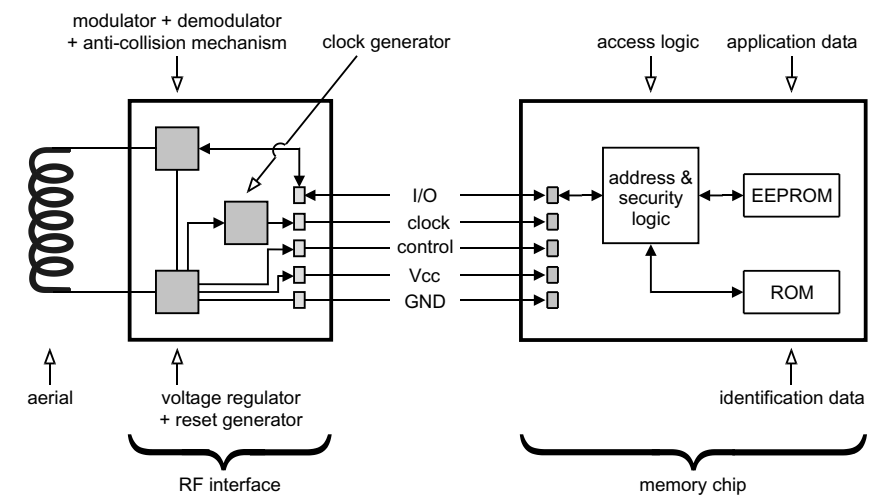
Figure 2.6 Typical architecture of a memory card with security logic and a contactless interface. The figure shows only basic energy and data flows and is not a detailed schematic diagram
