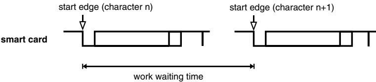
Figure 6.29 Definition of the work waiting time
