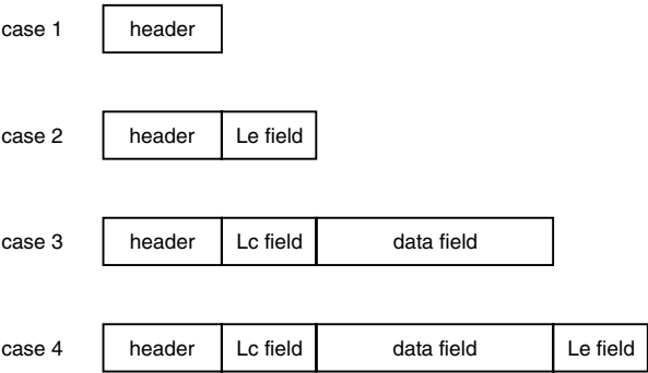
Figure 6.41 The four possible command APDU cases
