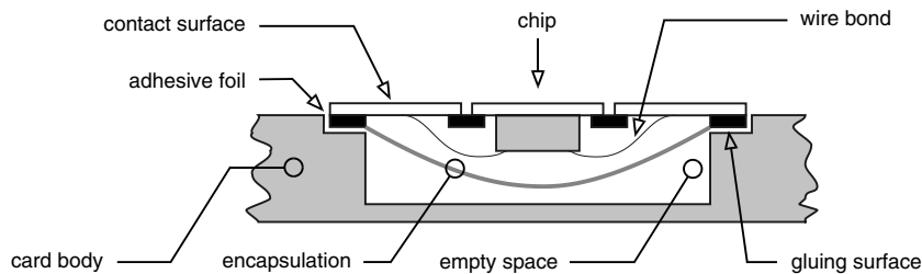
Figure 3.21 Cross-section of a chip-on-flex chip module
