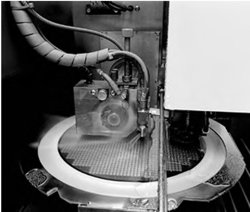
Figure 10.12 Sawing a wafer into dice ( Source: Renesas )
