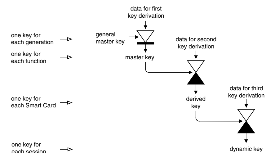
Figure 4.40 An example of a key hierarchy in a system based on smart cards and using symmetric cryptographic algorithms
