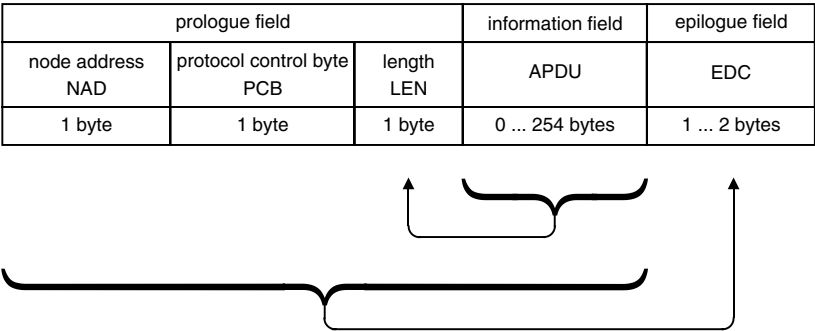
Figure 6.32 The structure of a T = 1 transmission block
