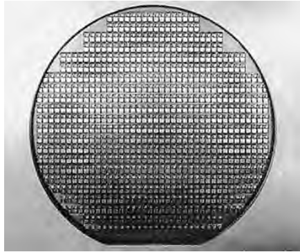
Figure 10.6 A 6-inch diameter wafer containing approximately 700 SLE44C80 microcontrollers. The milled straight edge (primary flat) is used to mark the orientation of the wafer during fabrication (Source: Infineon)
