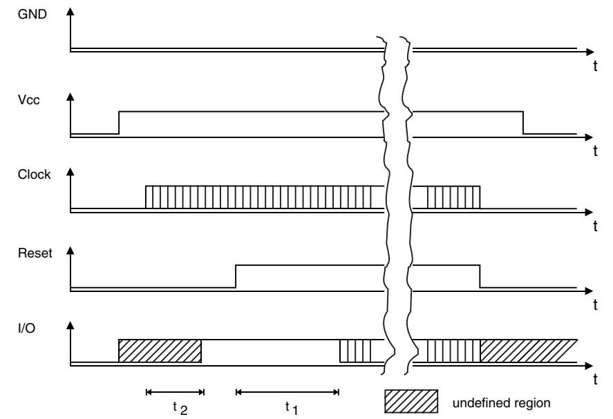
Figure 3.38 Smart card activation and deactivation sequences according to ISO/IEC 7816-3. The intervals t_1 and t_2 lie in the ranges 400/f \leq t_1 \leq 40,000/f and t_2 \leq 200/f
