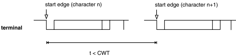
Figure 6.33 Definition of the character waiting time (CWT)
