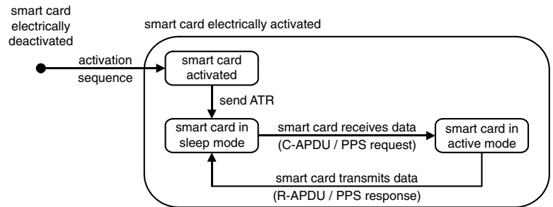
Figure 6.2 The general states of a smart card for activation and communication with the terminal
