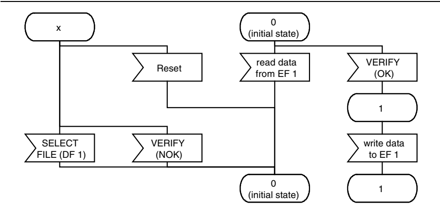
Figure 5.66 State diagram of the file with the FID '0001' (EF 1). Reading data from the EF and writing data to the EF relate to successful READ BINARY and UPDATE BINARY commands to the smart card, respectively. State 'x' is any arbitrary state
