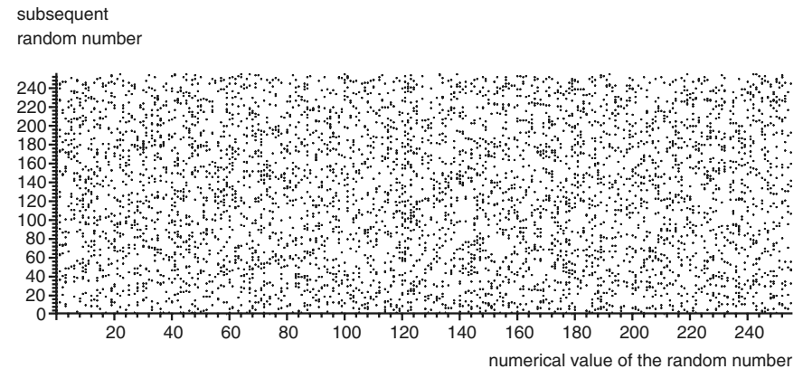
Figure 4.45 Graphic representation of the distribution of successor values of 5000 single-byte random numbers, corresponding to a spectral test. The nearly uniform distribution of the successor values can be seen at a glance from the regular pattern. The numbers were generated by a typical smart card pseudo-random number generator
