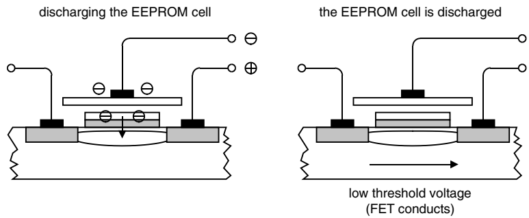
Figure 3.54 Discharging an EEPROM cell
