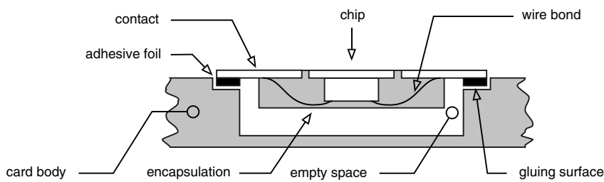
Figure 3.26 Cross-section through a lead-frame chip module
