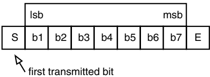
Figure 3.94 Structure of a short frame
