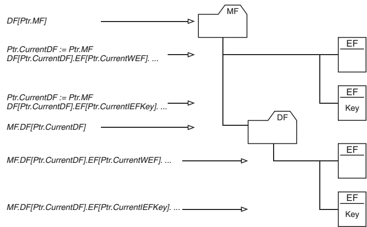
Figure 5.65 Example of the addressing of directories (MF and DF) and files (EFs) within the data structures available in Small-OS
