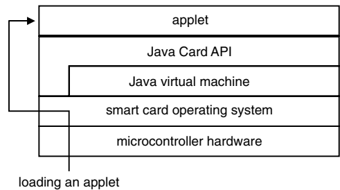
Figure 5.52 The basic process for loading an applet in a smart card operating system with Java
