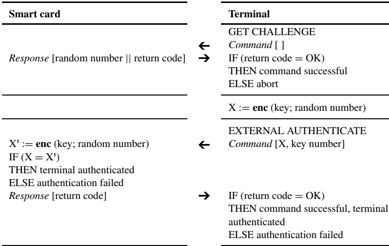
Figure 7.14 Sample command sequence using EXTERNAL AUTHENTICATE
