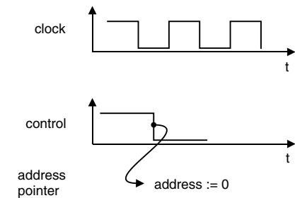
Figure 6.19 Resetting the address pointer to zero
