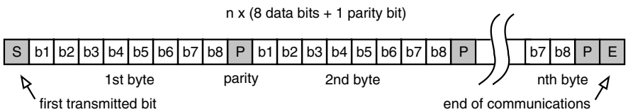
Figure 3.95 Structure of a standard frame
