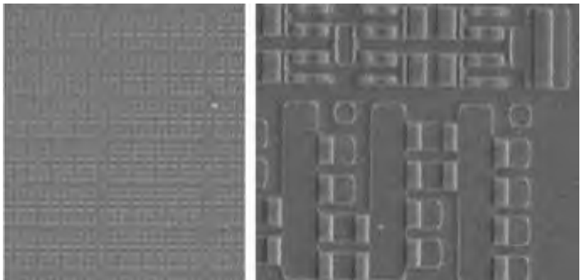
Figure 3.51 Photo of an EEPROM cell at 1000× enlargement (left) and 4000× enlargement (right) (Source: Giesecke & Devrient)
