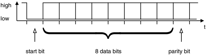
Figure 6.5 Structure of a character for data transmission
