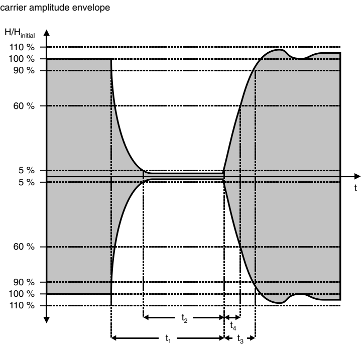
Figure 3.87 Specification of the blanking interval (gap) according to ISO/IEC 14433-2. The maximum duration of the gap is limited to 3 \mu\text{s} in order to interrupt the energy supply to the card as briefly as possible. Here 2.0 \mu\text{s} \leq t_1 \leq 3.0 \mu\text{s} ; 0.5 \mu\text{s} \leq t_2 \leq t_1 if t_1 > 2.5 \mu\text{s} , or 0.7 \mu\text{s} \leq t_2 \leq t_1 if t_1 \leq 2.5 \mu\text{s} ; and 0 \mu\text{s} \leq t_4 \leq 0.4 \mu\text{s}
