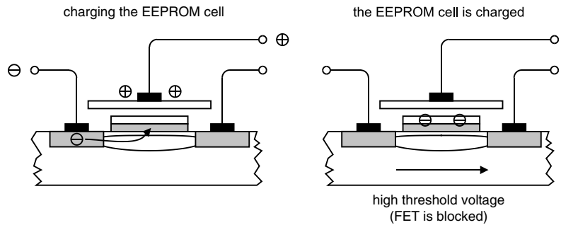
Figure 3.53 Charging an EEPROM cell
