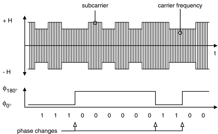
Figure 3.81 Operating principle of phase modulation for data transmission with a contactless smart card. The upper diagram shows the alternating magnetic field, and the associated phase states are shown in the lower diagram. The carrier frequency is 4.9152 MHz, and the subcarrier frequency is 307.2 kHz
