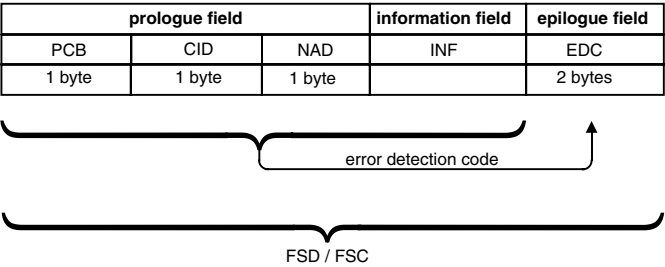
Figure 3.128 Block structure
