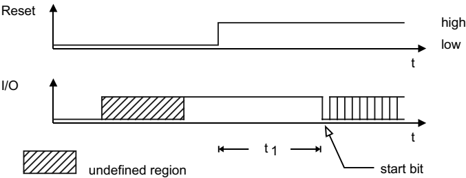
Figure 6.10 Timing diagram of the reset signal and the start of the ATR, in accordance with ISO/IEC 7816-3 (400 clock cycles \leq t_1 \leq 40,000 clock cycles)
