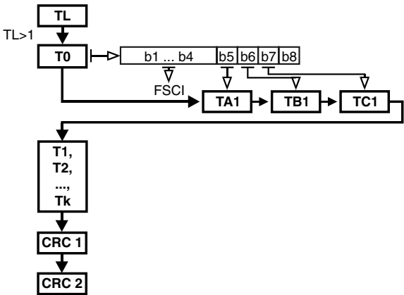
Figure 3.125 Format of ATS
