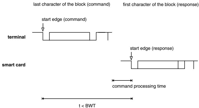
Figure 6.34 Definition of the block waiting time (BWT)
