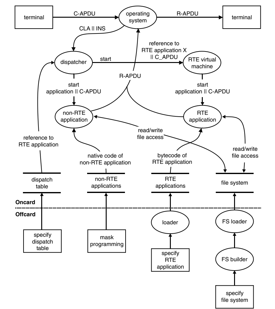
Figure 5.58 Data flow diagram for the essential components of Windows for Smart Cards. This diagram shows the fundamental IT relationships between these components. It has been produced based on published descriptions and makes no claim to being complete
