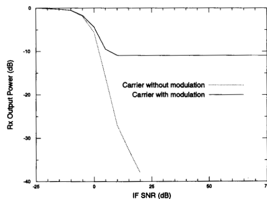
Fig. 1. Receiver output power versus IF S/N .
