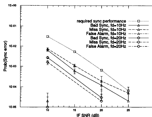
Fig. 20. Integrated system synchronization performance.
