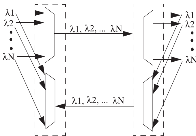
Figure 14-48. N-wavelength Point-to-Point WDM System
