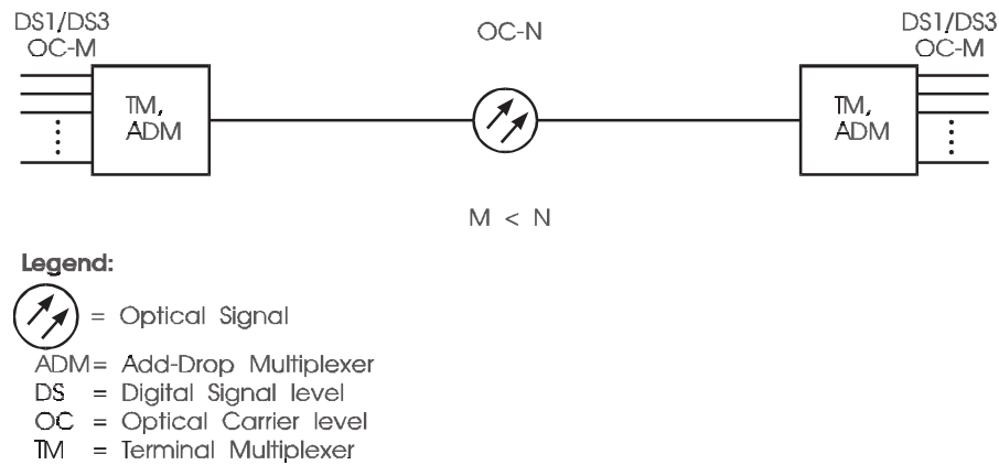
Figure 14-40. Point-to-Point Architecture
