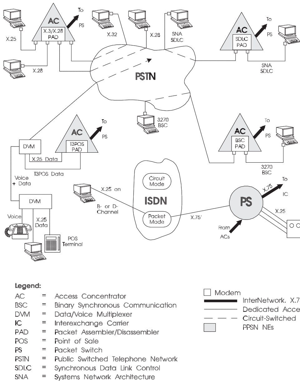
Figure 14-26. PPSN Access Interfaces
