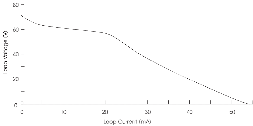
Figure 6-8. Loop Voltage Versus Current, 5ESS Line Circuit
