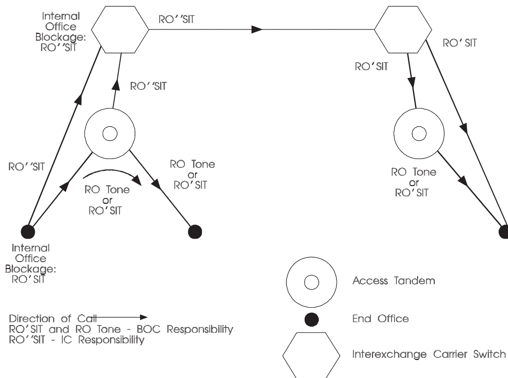
Figure 6-61. Reorder Condition
