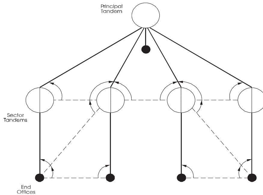
Figure4-8. Three-Level IntraLATA Network
