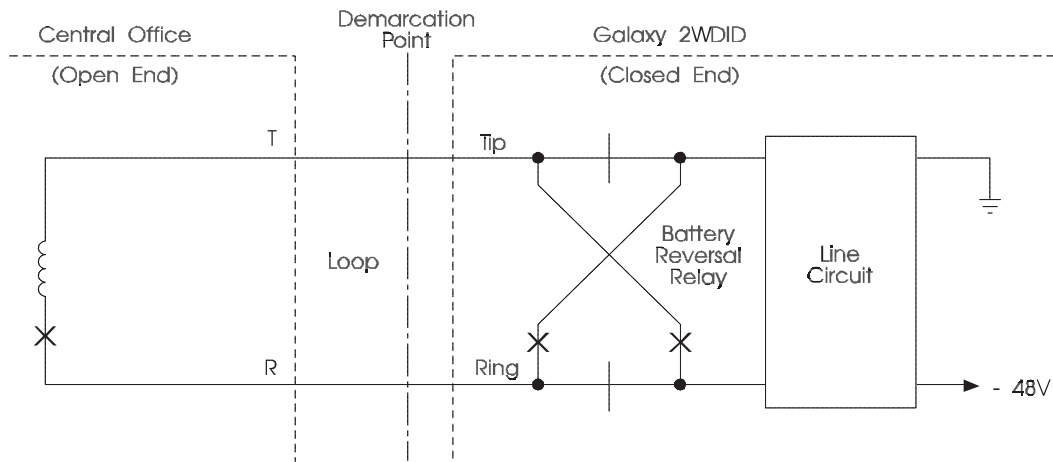
Figure 6-6. Loop Reverse-Battery Signaling for DID
