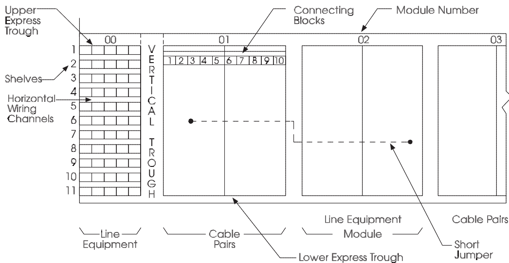
Figure 9-4. Modular Distributing Frame
