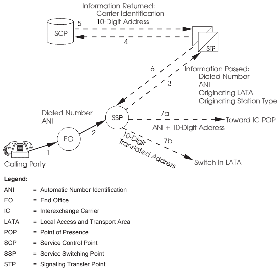
Figure 14-9. Current Toll-Free Network Configuration
