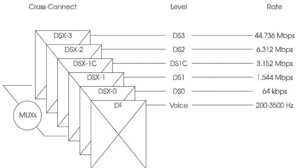
Figure 9-5. Interconnection Hierarchy
