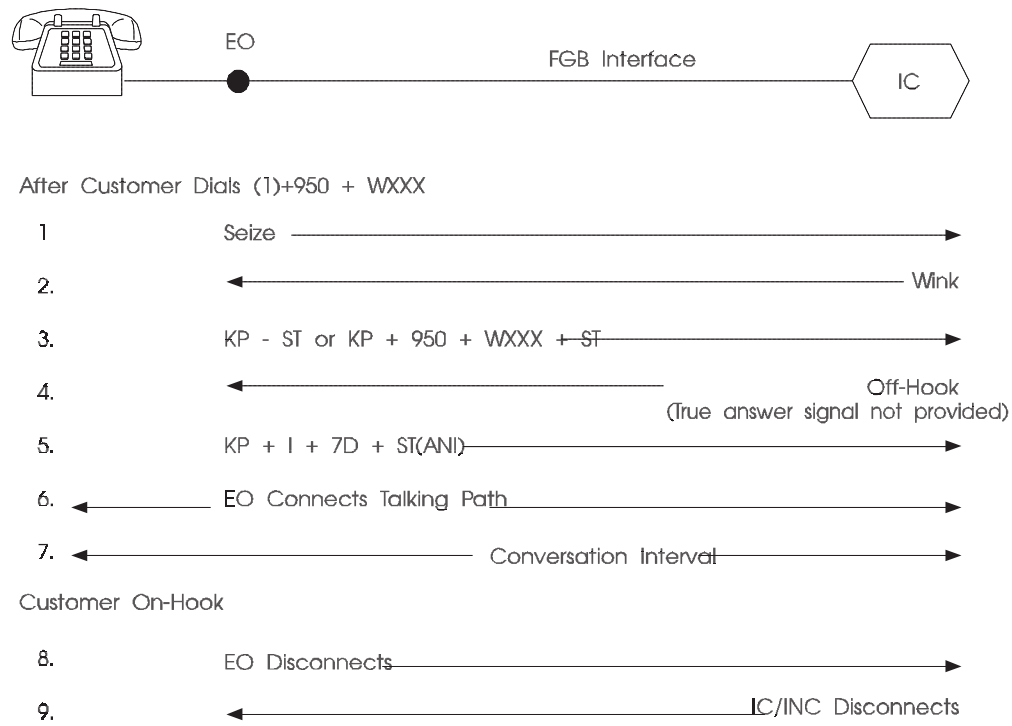
Figure 6-45. Originating Signaling Sequence — With ANI Direct Connection — FGB
