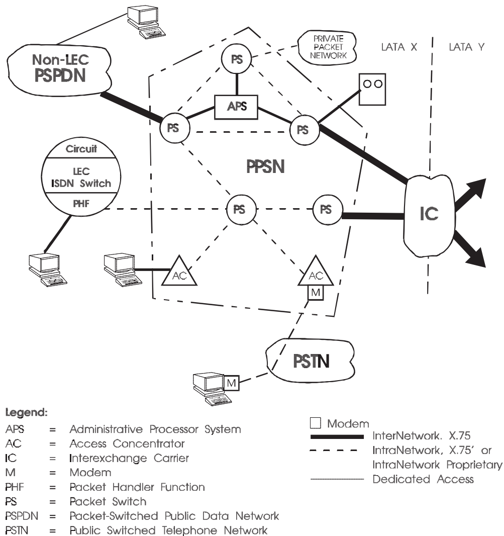
Figure 14-25. PPSN Architecture
