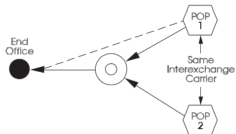
Figure 4-14. Terminating Routing
