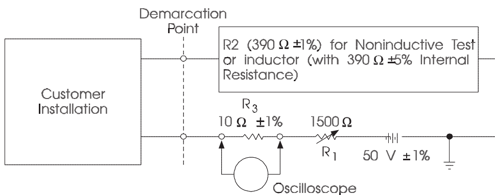
Figure 6-33. Test Circuit for Dial-Pulse Templates
