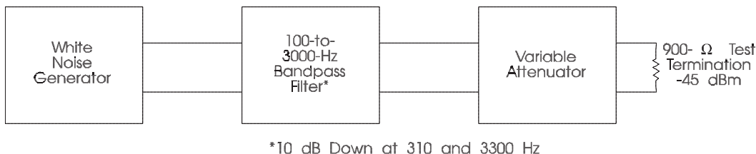
Figure 6-39. Gaussian Noise Source
