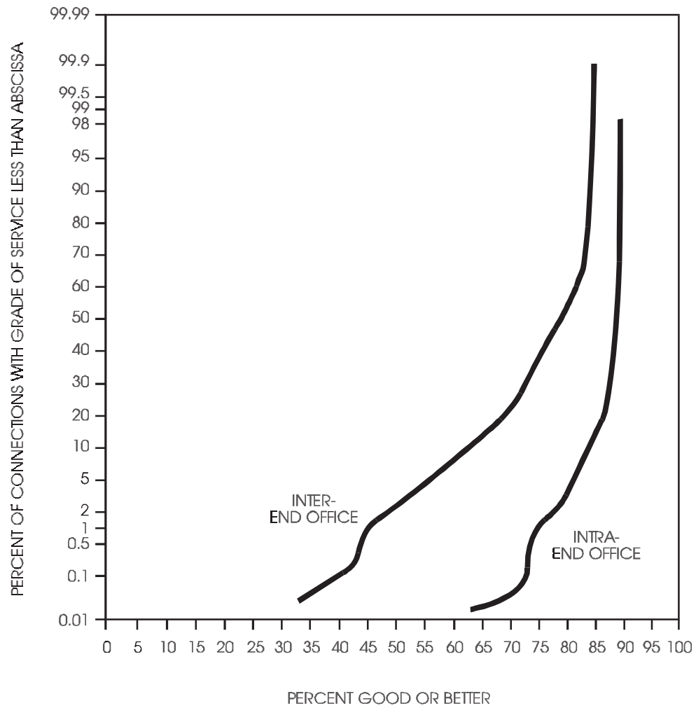
Figure 7-13. Grade-of-Service Distributions
