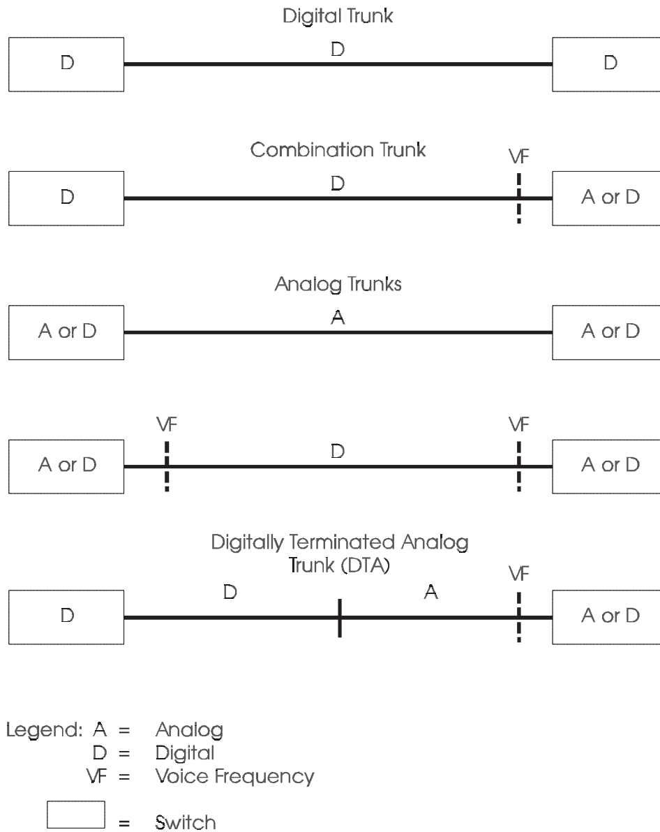
Figure 7-15. Trunk Types
