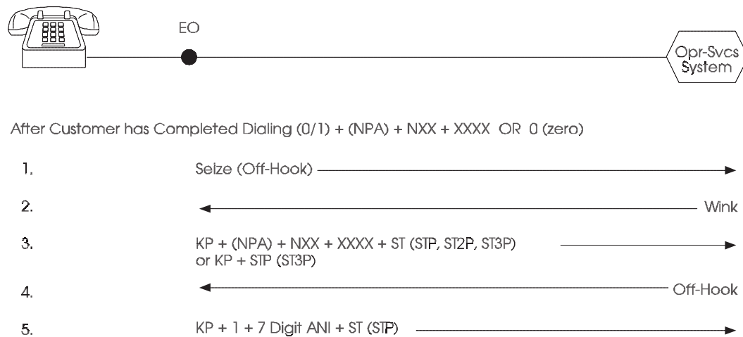
Figure 6-58. Originating Signaling Sequence
