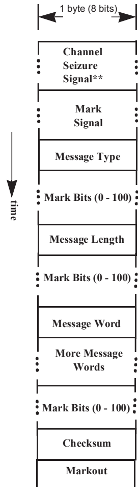
Single Data Message Frame Format
