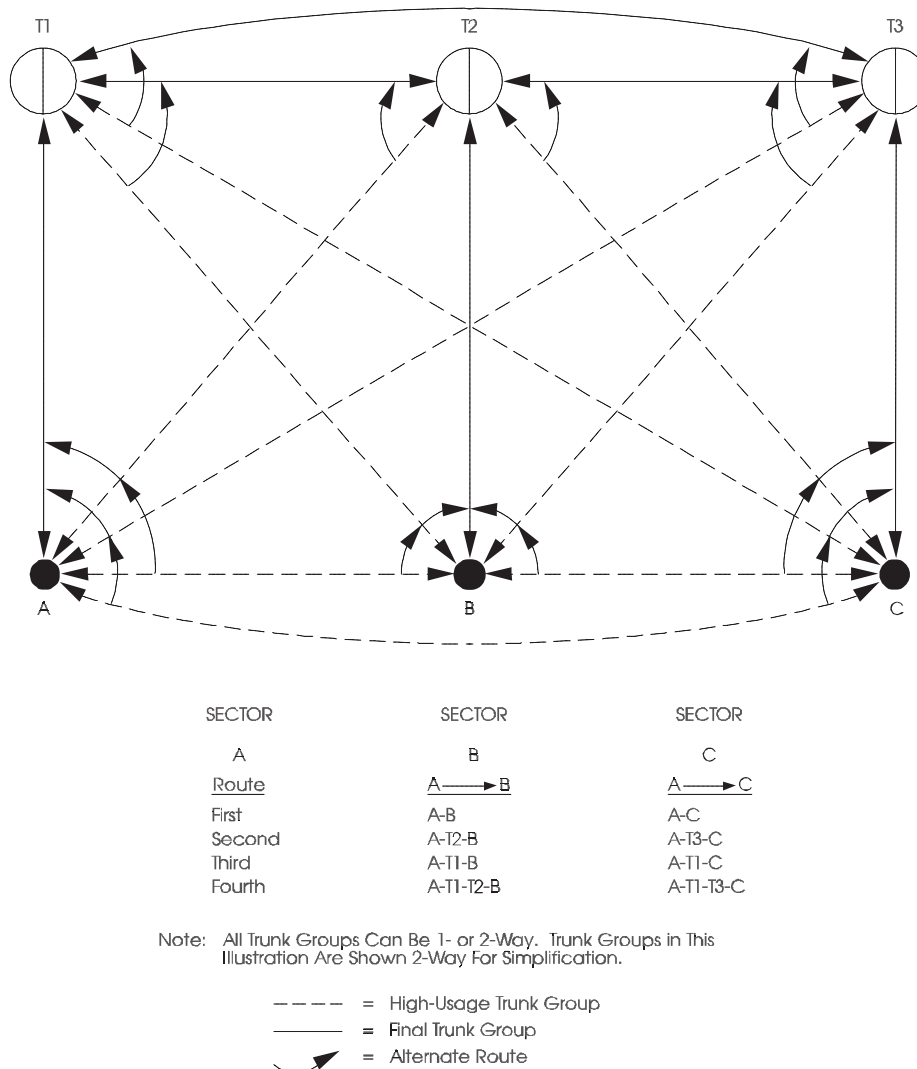
Figure 4-7. Combined Sector-Tandem Configuration with Multistage Alternate Routing
