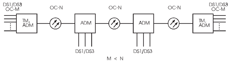
Figure 14-41. Linear Architecture
