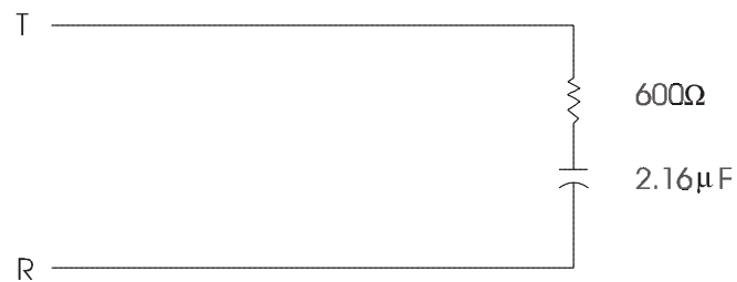
Figure 8-3. 600-Ω Quiet Termination
