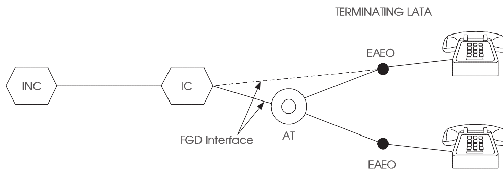
Figure 6-55. INC Interconnection — Indirect — Terminating LATA — FGD
