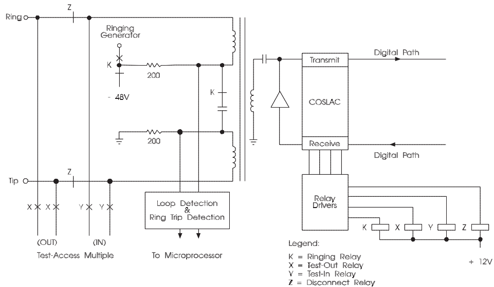
Figure 6-11. EWSD Switching System — Single-Party Line Circuit
