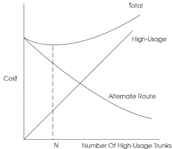
Figure4-4. Relationships Involved in Alternate Routing Arrangement
