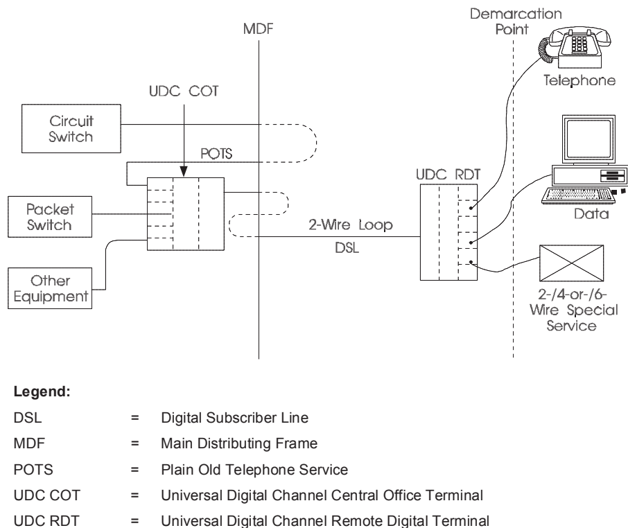
Figure 12-26. Universal Digital Channel
