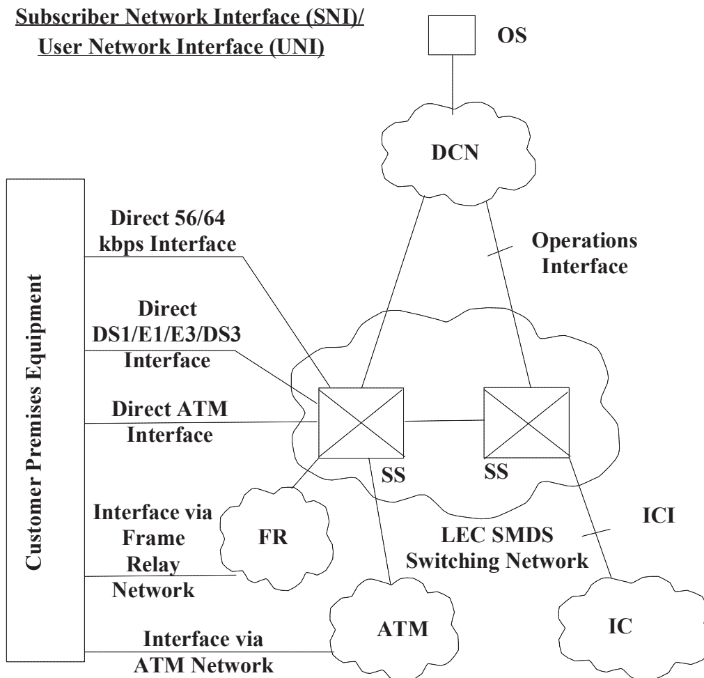
Figure 14-31. Example of Networks in Support of SMDS
