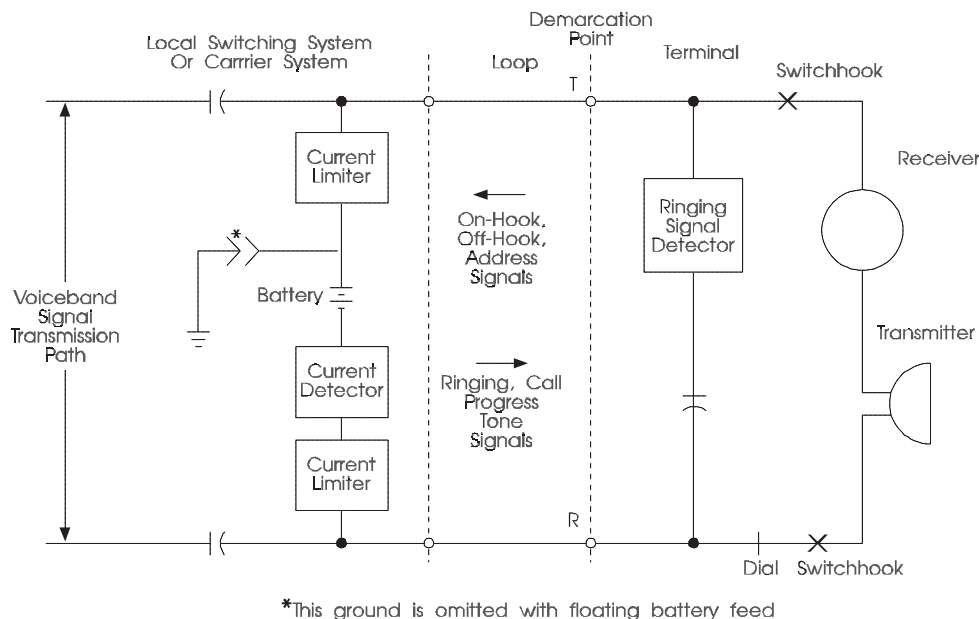
Figure 6-1. Principle of Operations of Loop-Start Signaling
