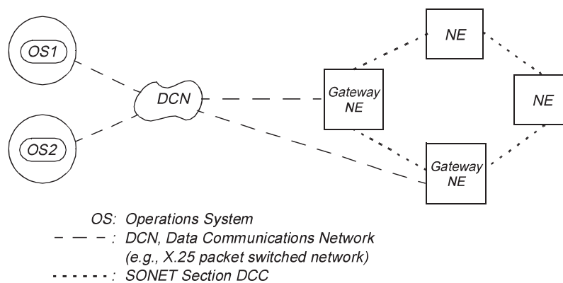
Figure 14-57. Example Operations Communications Network for a Survivable Ring
