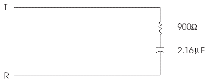
Figure 8-2. 900-Ω Quiet Termination
