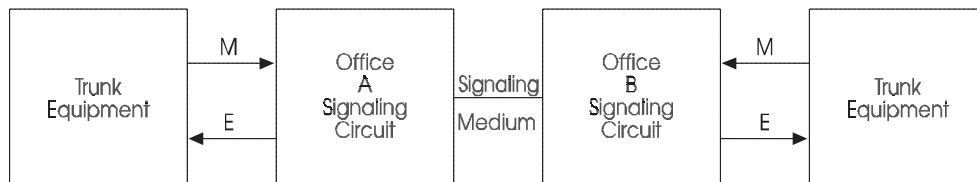
Figure 6-16. E&M Lead Control Status
