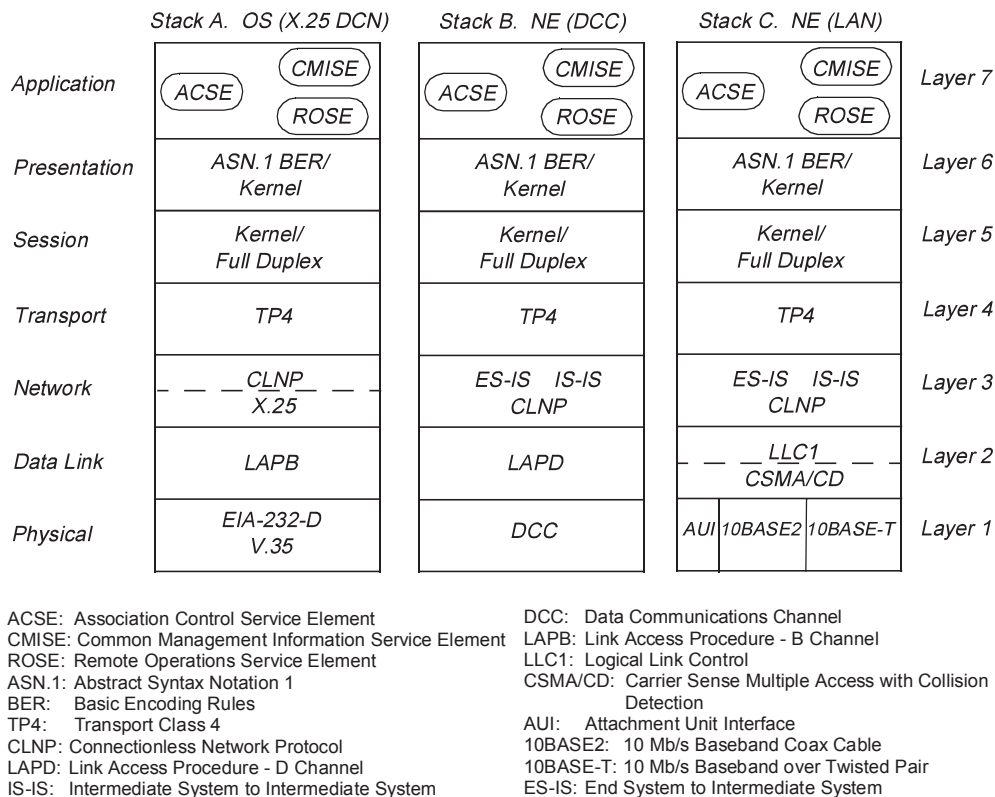
Figure 14-55. Interactive Protocol Stacks for SONET Operations Communications
