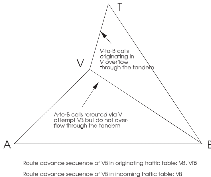
Figure 4-18. Restricting DRT to Two-Link Paths
