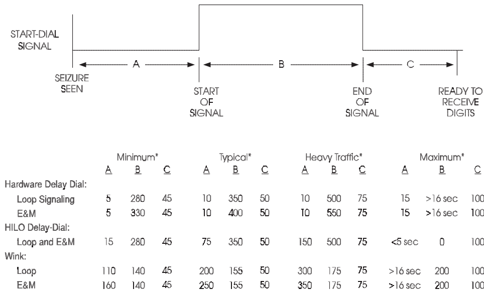
Figure 6-13. Controlled-Outpulsing Formats for 1/1A ESS Systems
