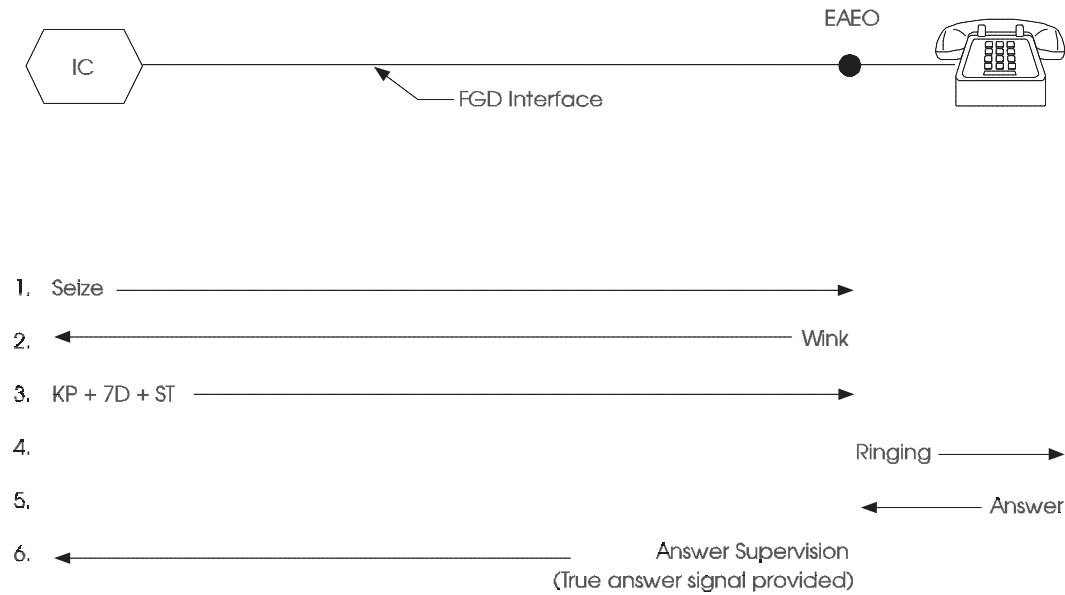
Figure 6-53. Terminating Sequence — Direct From IC to EAE0 Tandem — FGD
