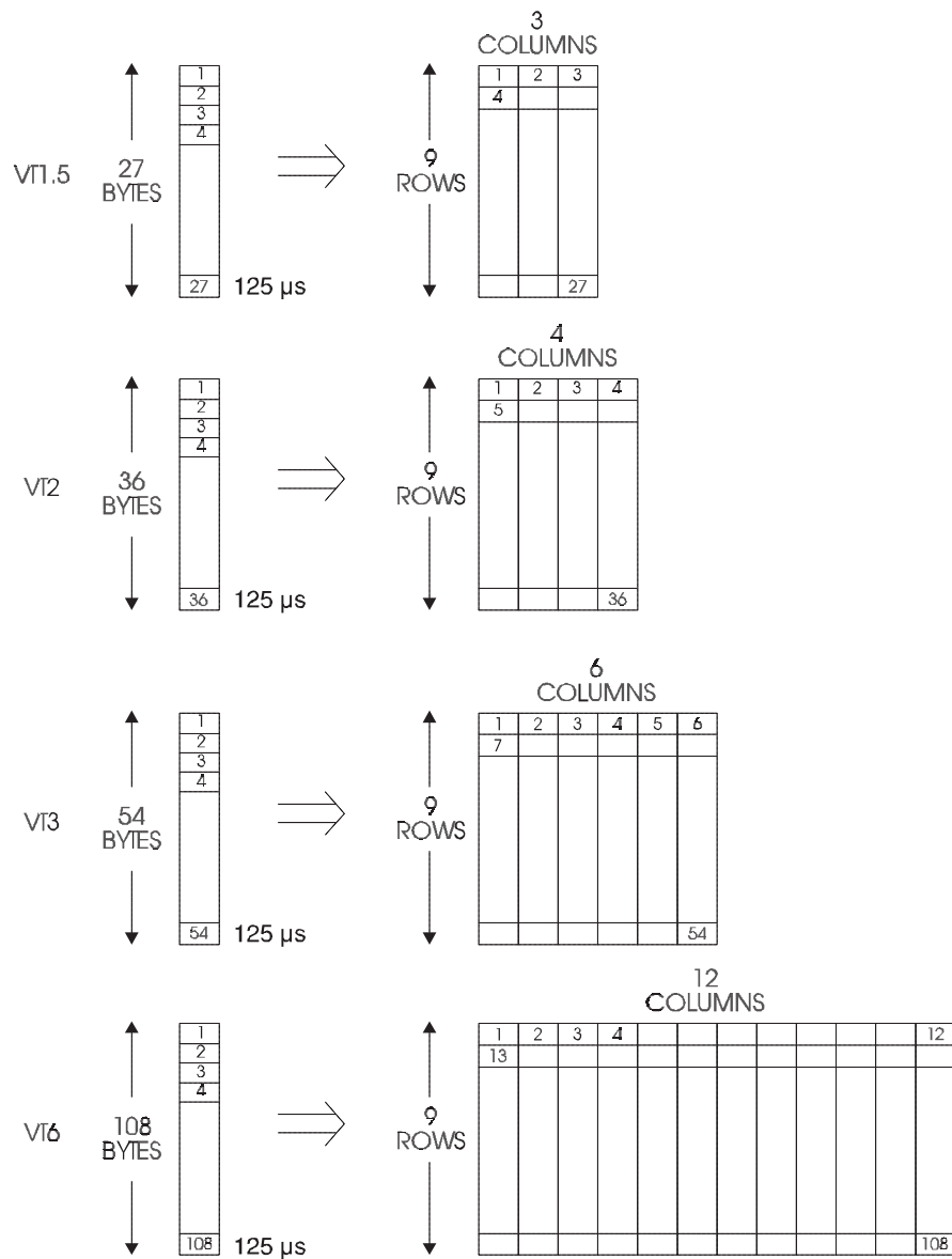
Figure 14-37. VT Sizes
