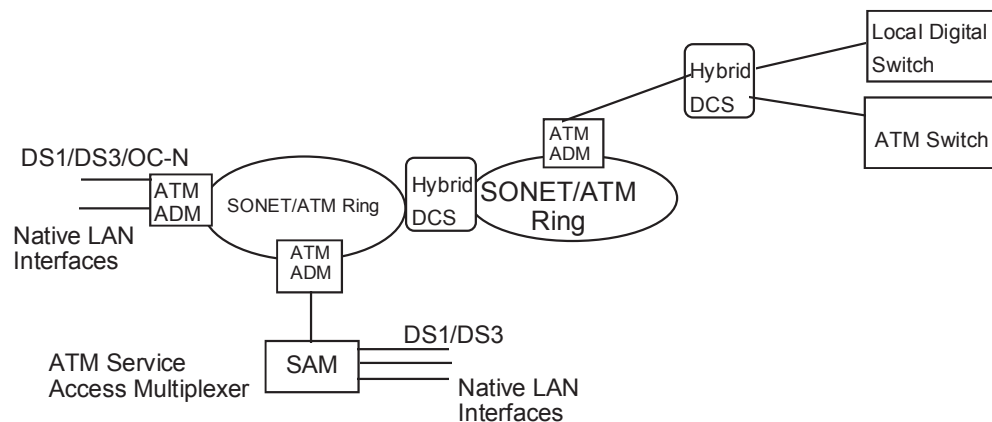
Figure 14-51. Hybrid SONET/ATM NEs in an Example Network
