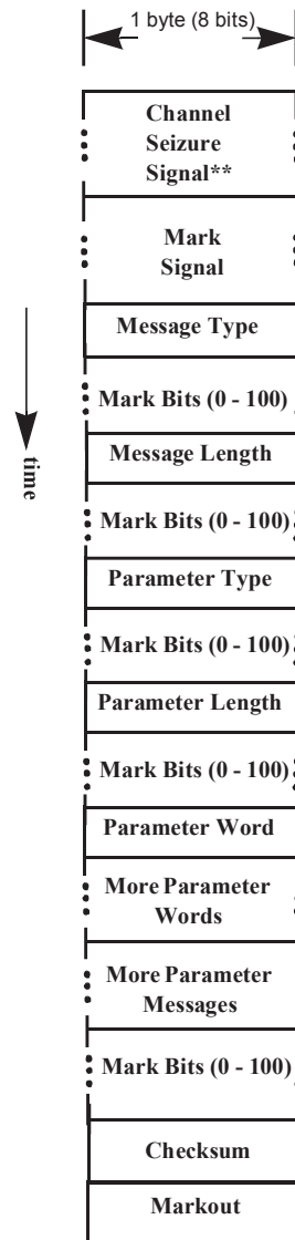
Multiple Data Message Frame Format
