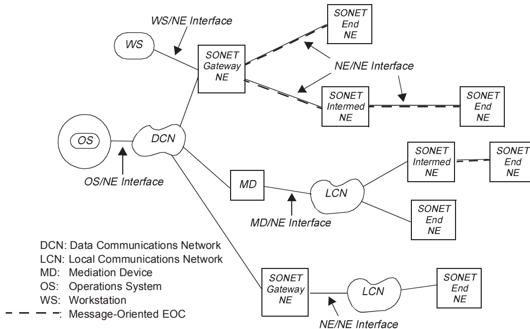
Figure 14-53. SONET Operations Communication: Example NE and Interface Types
