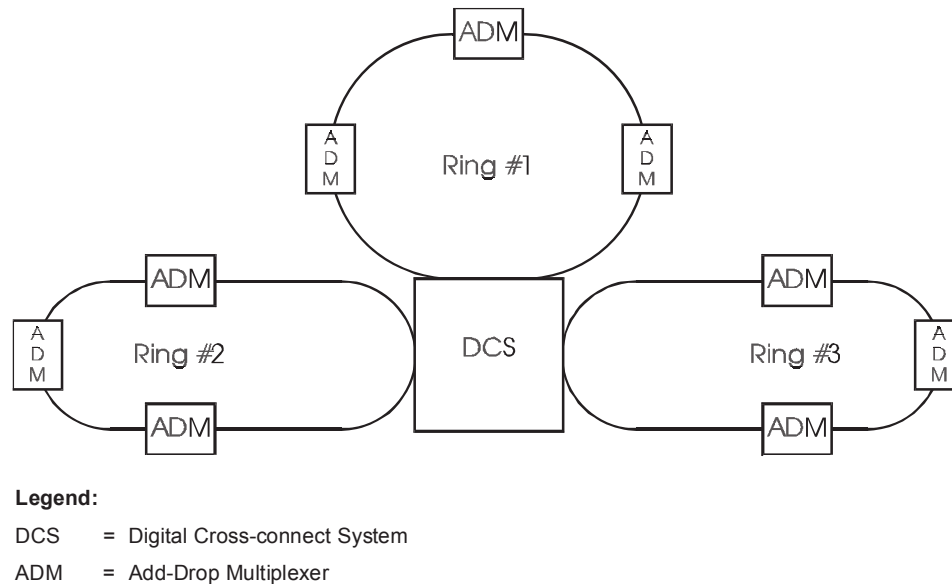
Figure 14-47. DCS Ring Architecture (Single Homing)
