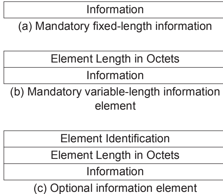
Figure 6-68. ISUP — Information Element Format
