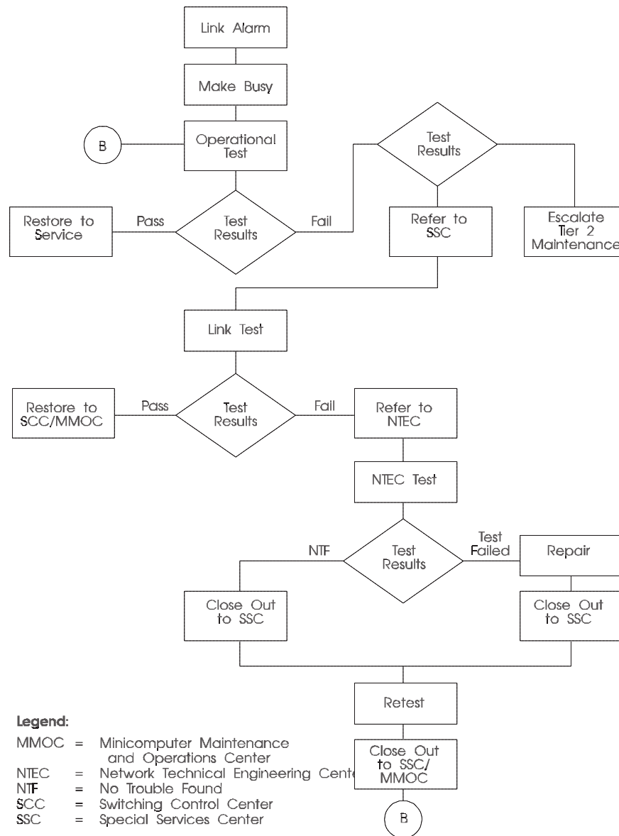
Figure 8-19. Example of Link Maintenance Flow
