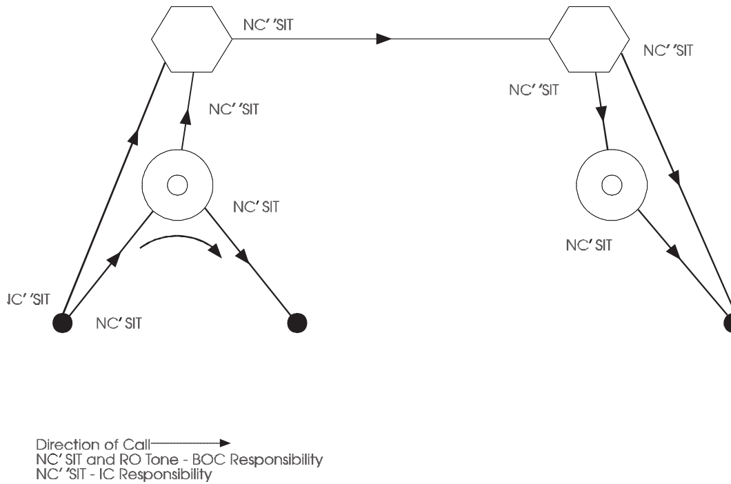
Figure 6-62. No-Circuit Condition
