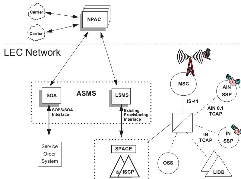
Figure 14-18. Bellcore INS Solution for Number Portability
