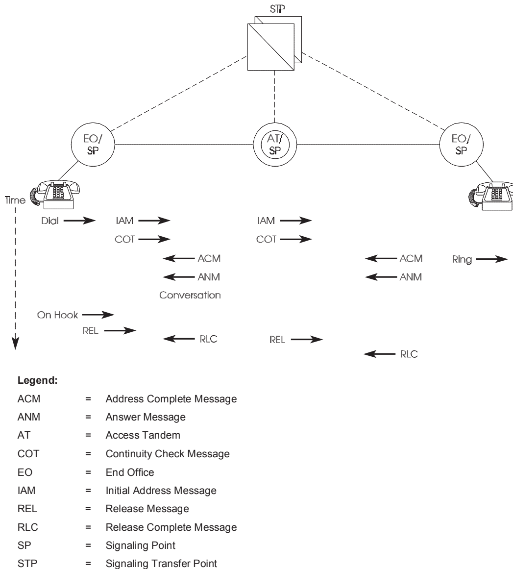
Figure 14-4. CCS IntraLATA Call Setup
