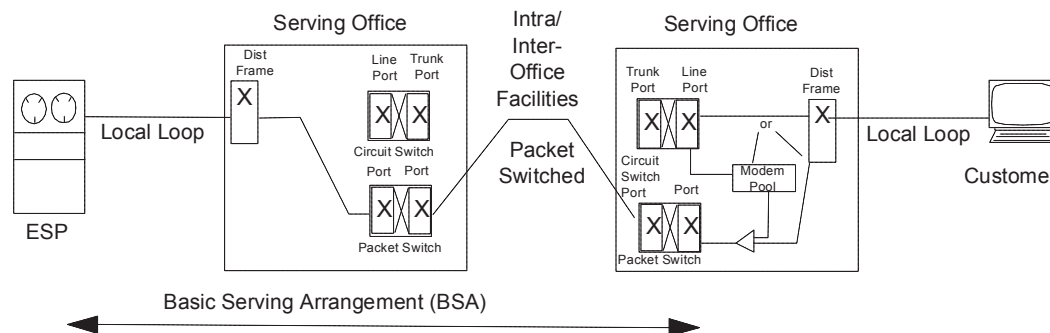
Figure 17-4. Packet Switching BSA
