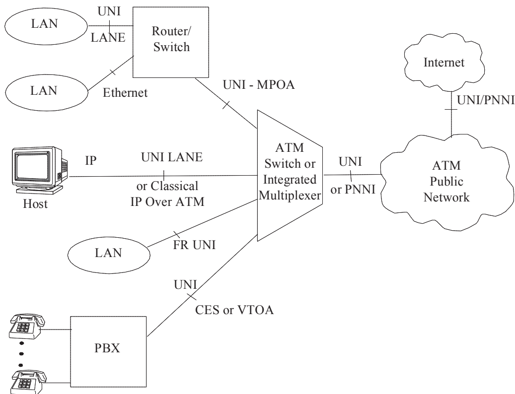
Figure 14-37. Campus/Enterprise Environment
