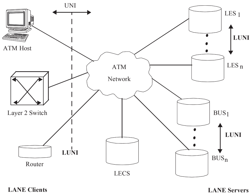
Figure 14-36. LANE Components
