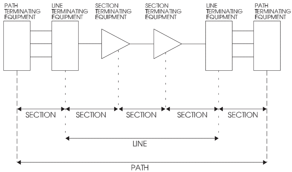
Figure 14-38. Simplified Diagram Depicting SONET Section, Line, and Path Definitions
