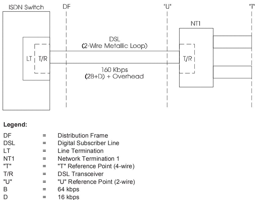
Figure 12-20. ISDN Basic Rate Access Configuration
