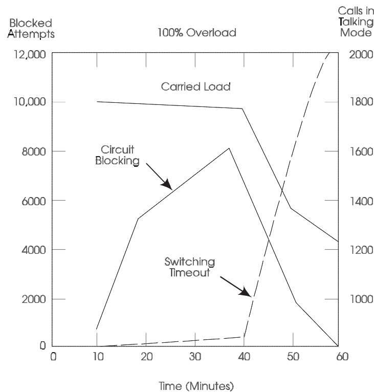
Figure 10-2. Network Congestion
