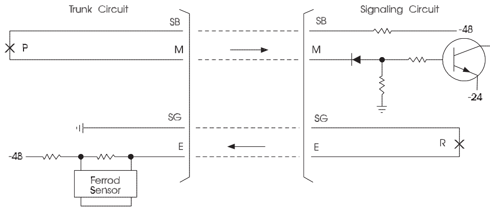
Figure 6-18. Type II Interface
