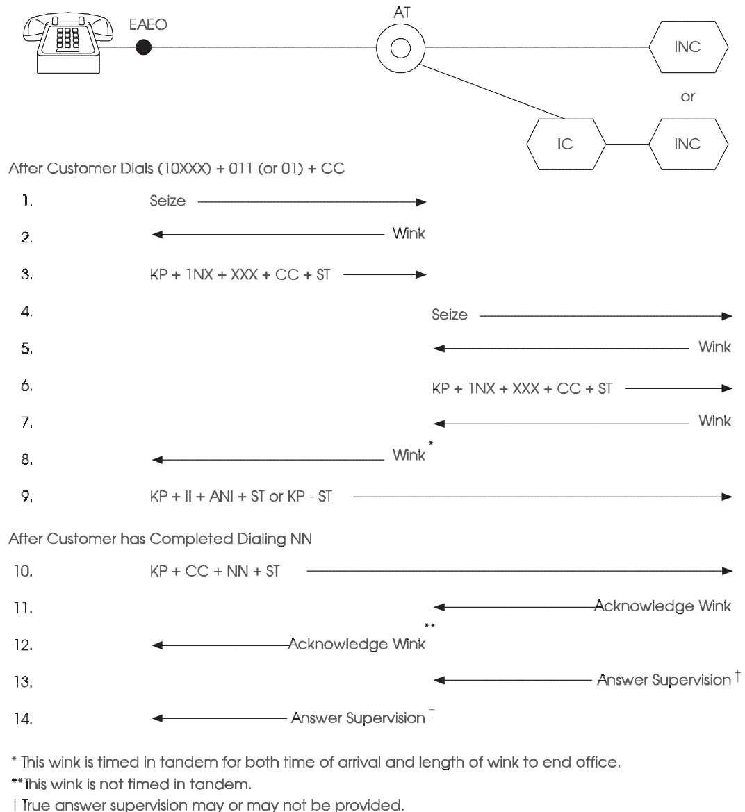
Figure 6-56. International Call - Originating Signaling Sequence at Connection to INC (or via IC) — FGD
