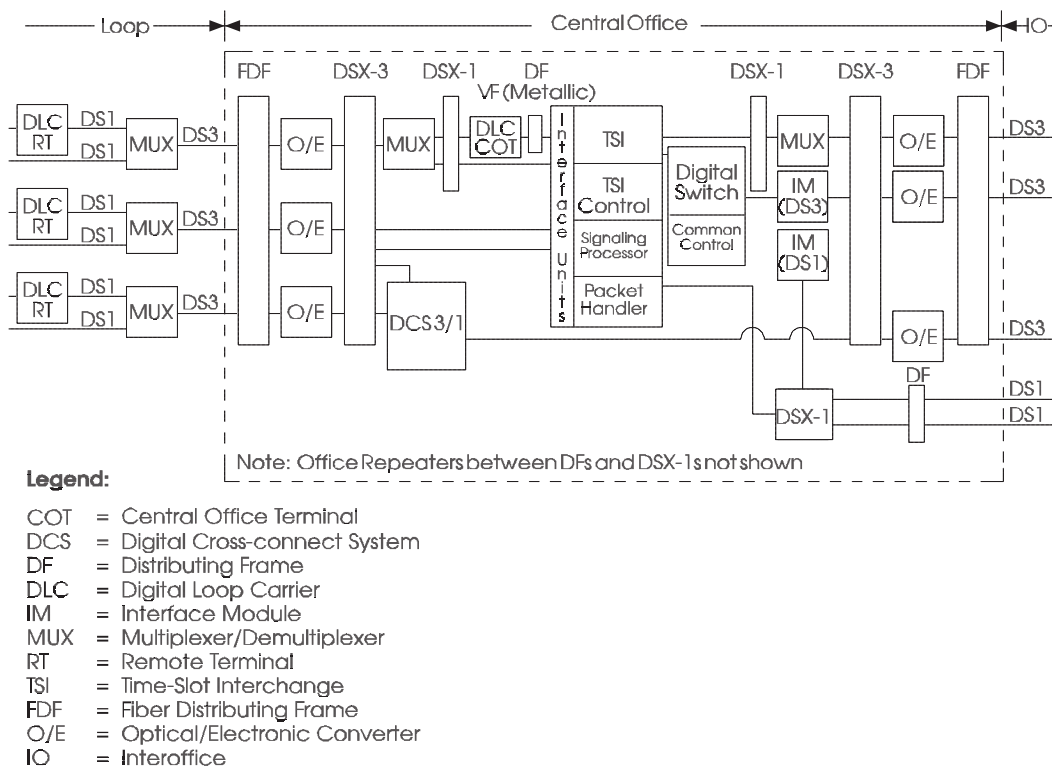
Figure 9-6. Central Office Cross-Connect Network
